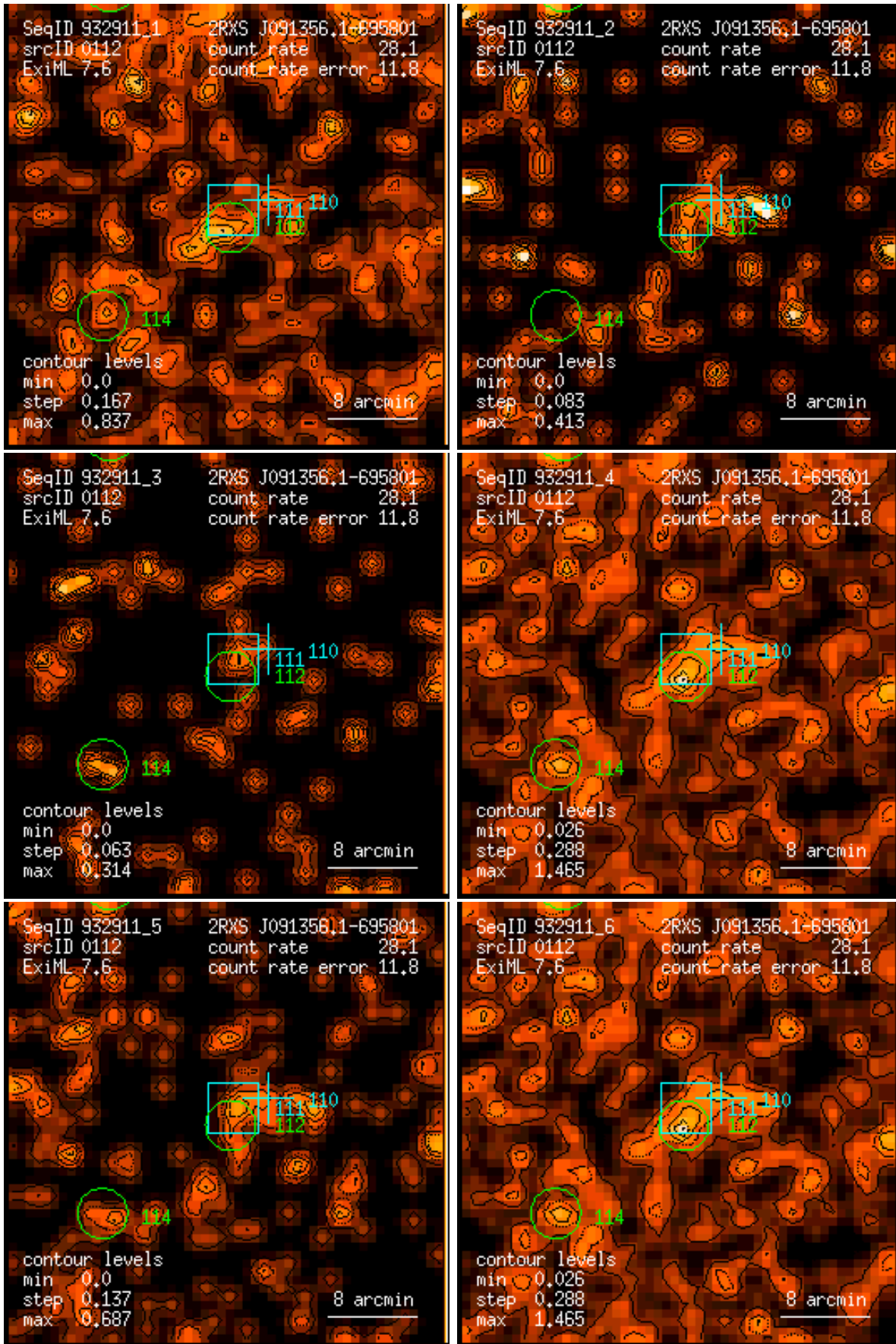
Figure 112: RASS 932911: detection 0112: band rate images, Gaussian filter: (1) PSPC channels 11 – 41, (2) 52 – 90, (3) 91 – 201, (4) 11 – 235, (5) 52 – 201, (6) 11 – 201. Broad band rates in counts/ks. Band rate contour levels in counts/ks/arcmin 2 .
