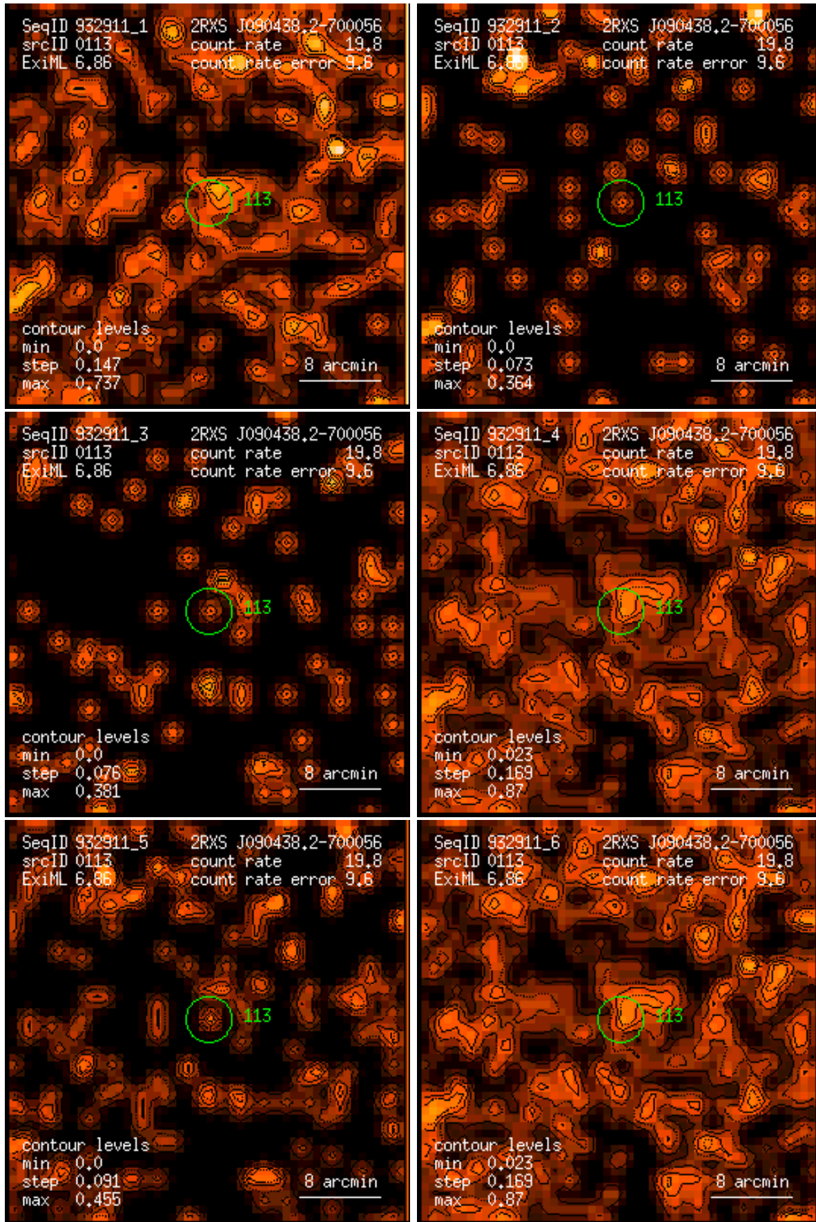
Figure 113: RASS 932911: detection 0113: band rate images, Gaussian filter: (1) PSPC channels 11 – 41, (2) 52 – 90, (3) 91 – 201, (4) 11 – 235, (5) 52 – 201, (6) 11 – 201. Broad band rates in counts/ks. Band rate contour levels in counts/ks/arcmin 2 .
