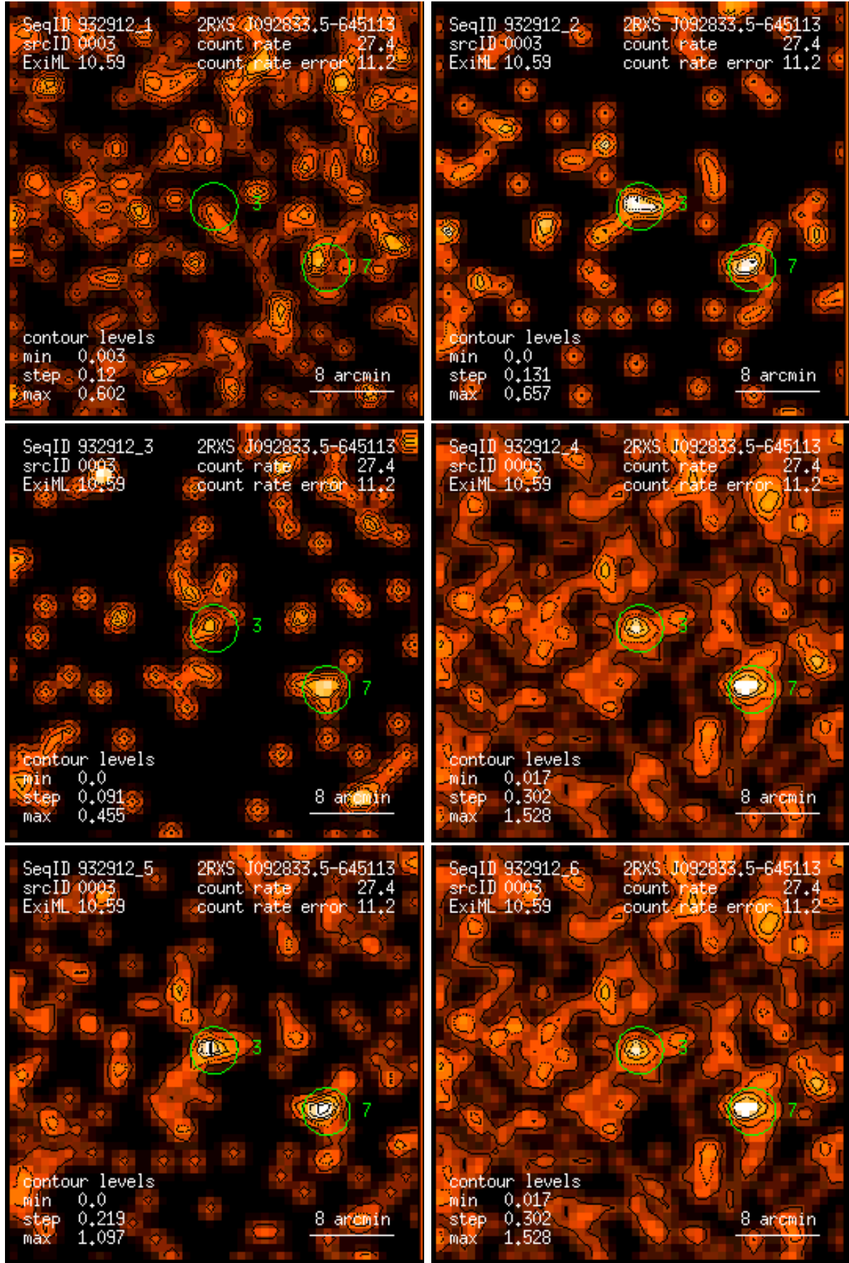
Figure 3: RASS 932912: detection 0003: band rate images, Gaussian filter: (1) PSPC channels 11 – 41, (2) 52 – 90, (3) 91 – 201, (4) 11 – 235, (5) 52 – 201, (6) 11 – 201. Broad band rates in counts/ks. Band rate contour levels in counts/ks/arcmin 2 .
