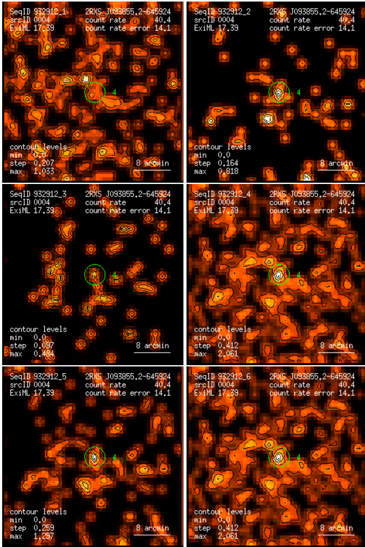
Figure 4: RASS 932912: detection 0004: band rate images, Gaussian filter: (1) PSPC channels 11 – 41, (2) 52 – 90, (3) 91 – 201, (4) 11 – 235, (5) 52 – 201, (6) 11 – 201. Broad band rates in counts/ks. Band rate contour levels in counts/ks/arcmin 2 .
