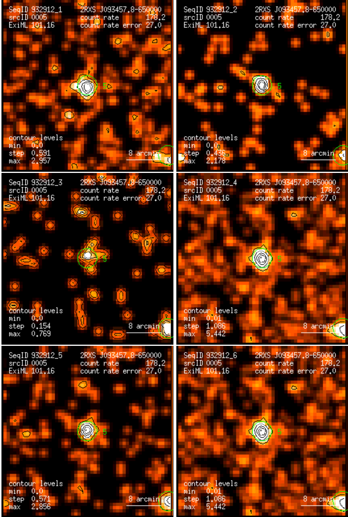
Figure 5: RASS 932912: detection 0005: band rate images, Gaussian filter: (1) PSPC channels 11 – 41, (2) 52 – 90, (3) 91 – 201, (4) 11 – 235, (5) 52 – 201, (6) 11 – 201. Broad band rates in counts/ks. Band rate contour levels in counts/ks/arcmin 2 .
