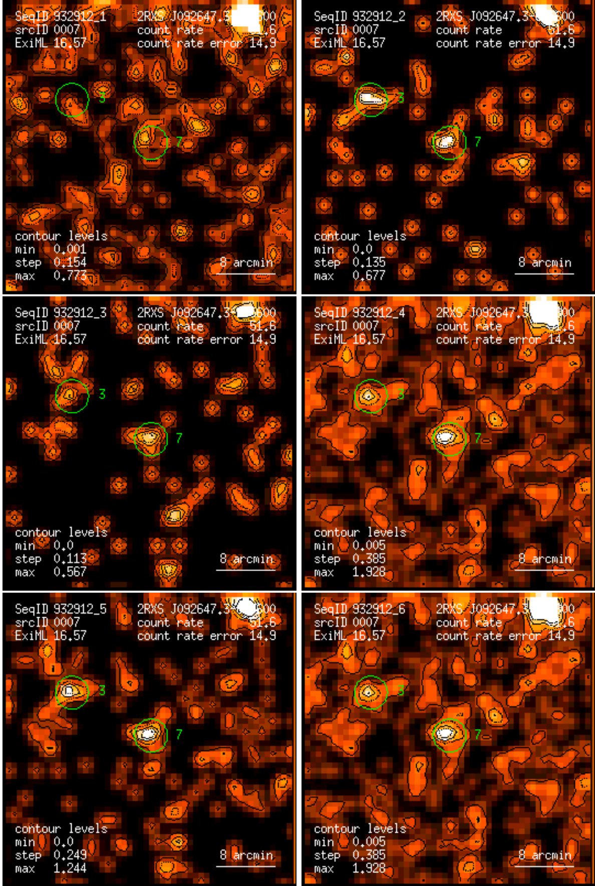
Figure 7: RASS 932912: detection 0007: band rate images, Gaussian filter: (1) PSPC channels 11 – 41, (2) 52 – 90, (3) 91 – 201, (4) 11 – 235, (5) 52 – 201, (6) 11 – 201. Broad band rates in counts/ks. Band rate contour levels in counts/ks/arcmin 2 .
