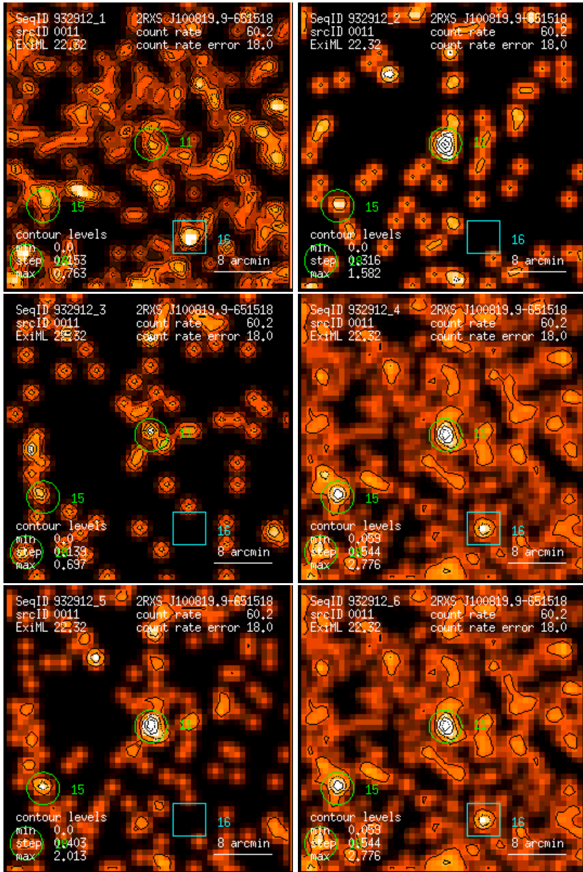
Figure 11: RASS 932912: detection 0011: band rate images, Gaussian filter: (1) PSPC channels 11 – 41, (2) 52 – 90, (3) 91 – 201, (4) 11 – 235, (5) 52 – 201, (6) 11 – 201. Broad band rates in counts/ks. Band rate contour levels in counts/ks/arcmin 2 .
