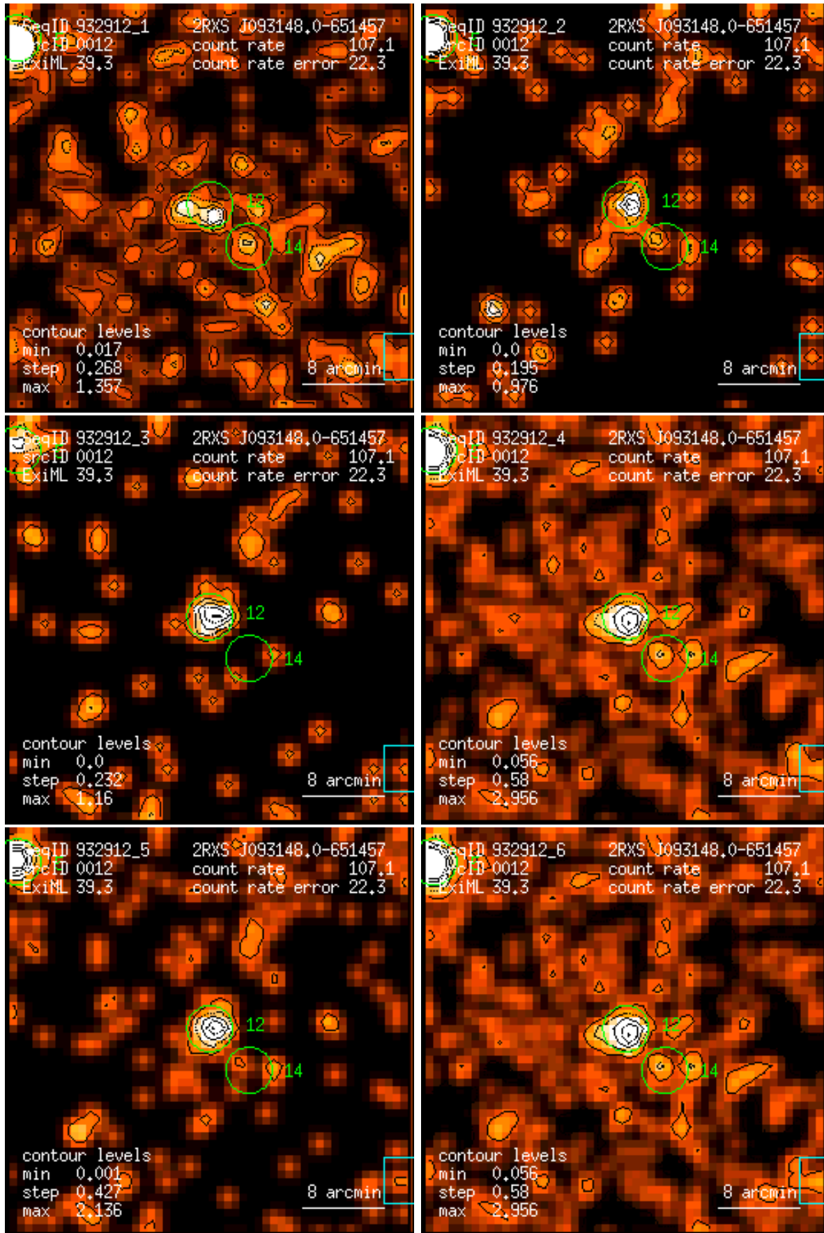
Figure 12: RASS 932912: detection 0012: band rate images, Gaussian filter: (1) PSPC channels 11 – 41, (2) 52 – 90, (3) 91 – 201, (4) 11 – 235, (5) 52 – 201, (6) 11 – 201. Broad band rates in counts/ks. Band rate contour levels in counts/ks/arcmin 2 .
