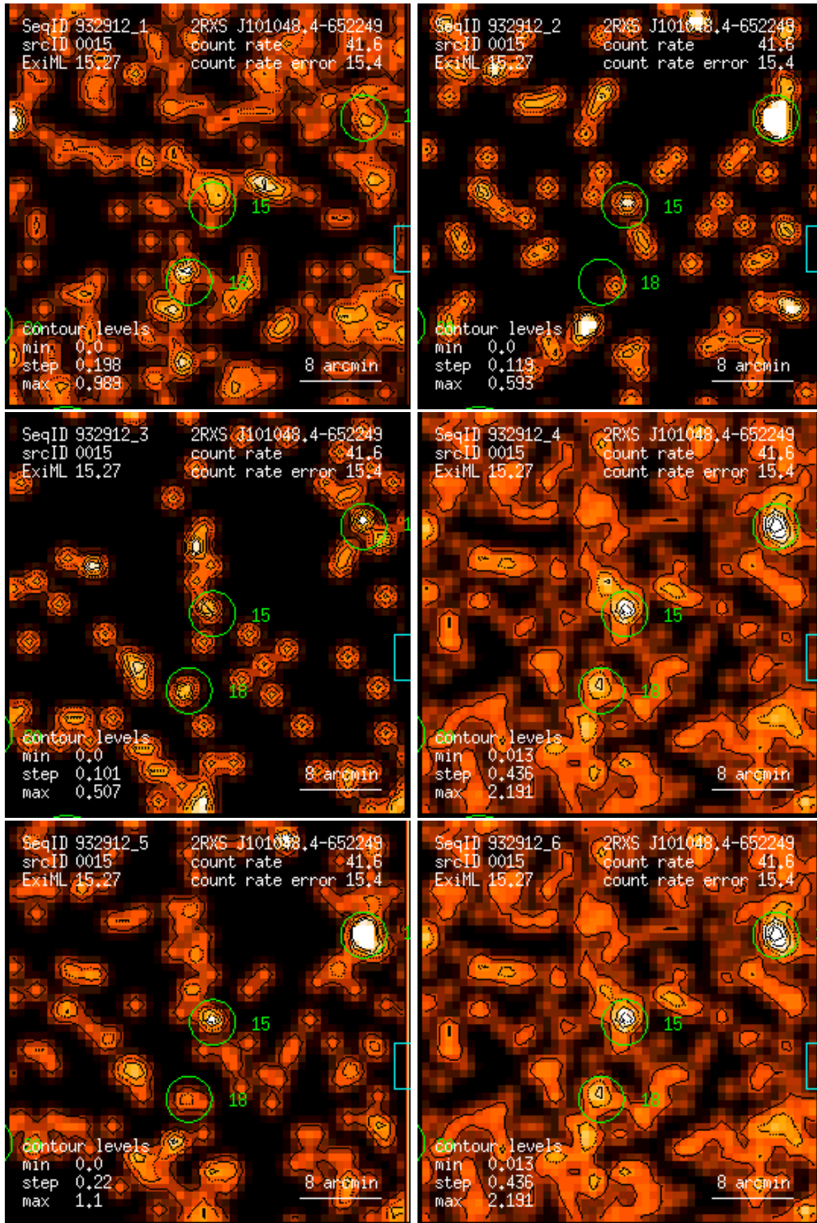
Figure 15: RASS 932912: detection 0015: band rate images, Gaussian filter: (1) PSPC channels 11 – 41, (2) 52 – 90, (3) 91 – 201, (4) 11 – 235, (5) 52 – 201, (6) 11 – 201. Broad band rates in counts/ks. Band rate contour levels in counts/ks/arcmin 2 .
