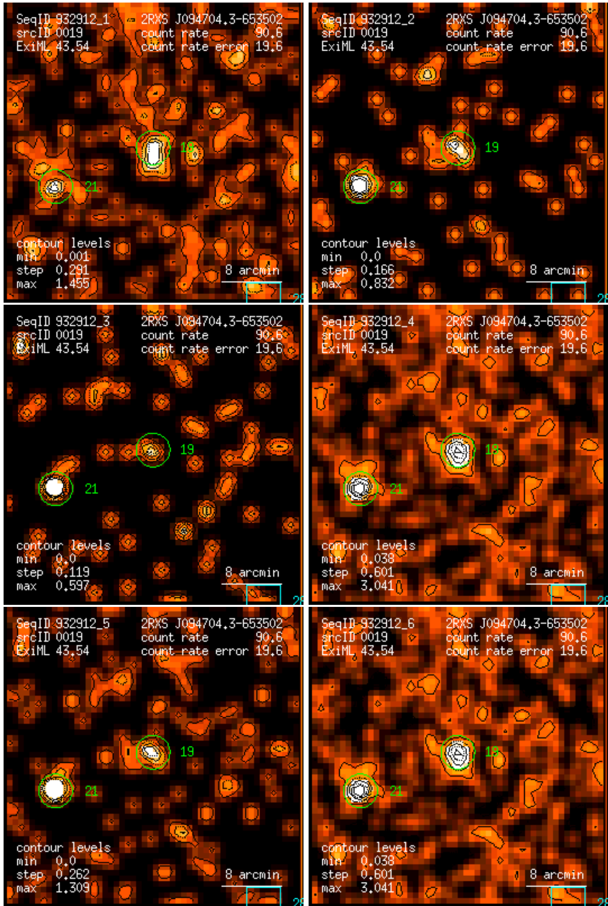
Figure 19: RASS 932912: detection 0019: band rate images, Gaussian filter: (1) PSPC channels 11 – 41, (2) 52 – 90, (3) 91 – 201, (4) 11 – 235, (5) 52 – 201, (6) 11 – 201. Broad band rates in counts/ks. Band rate contour levels in counts/ks/arcmin 2 .
