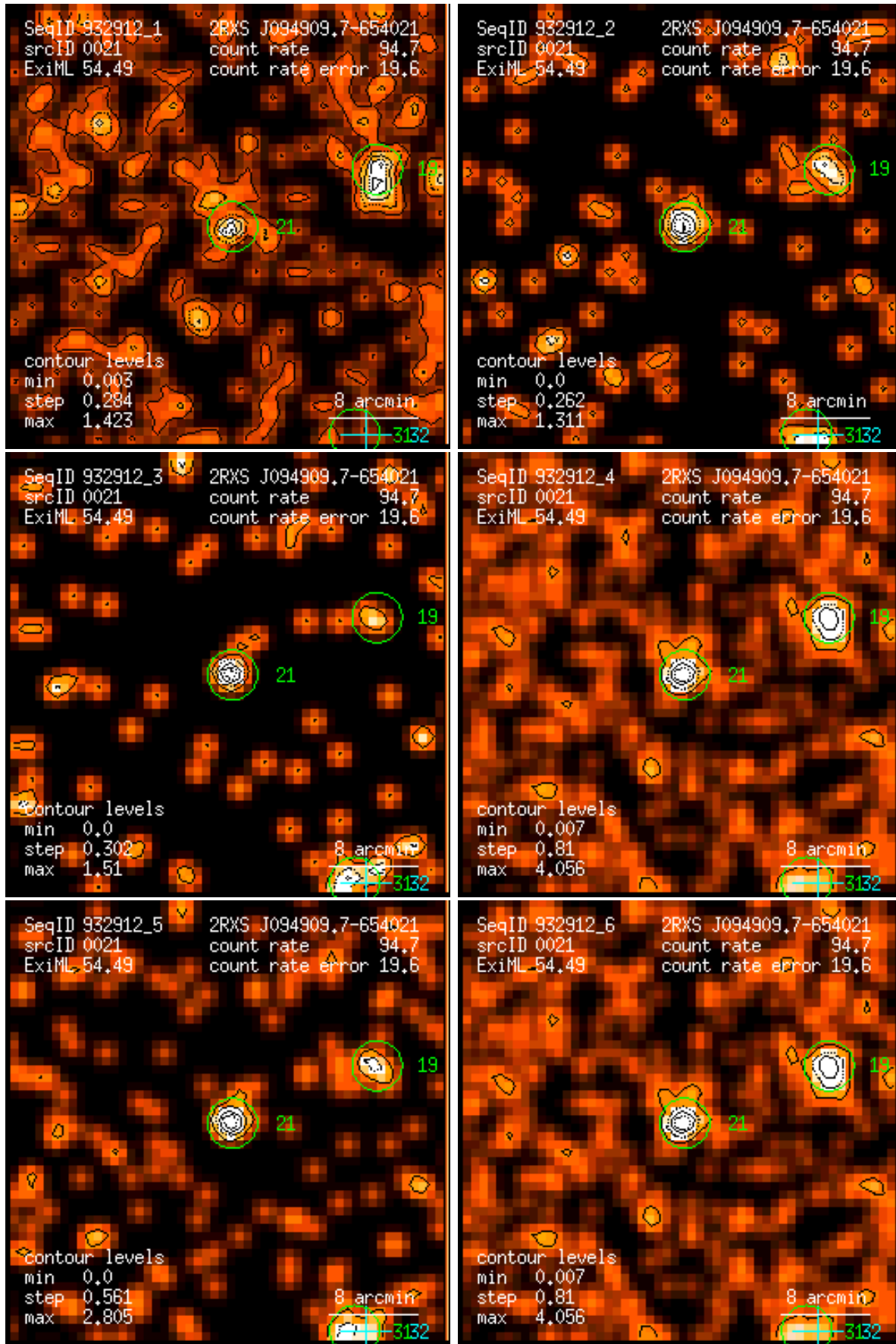
Figure 21: RASS 932912: detection 0021: band rate images, Gaussian filter: (1) PSPC channels 11 – 41, (2) 52 – 90, (3) 91 – 201, (4) 11 – 235, (5) 52 – 201, (6) 11 – 201. Broad band rates in counts/ks. Band rate contour levels in counts/ks/arcmin 2 .
