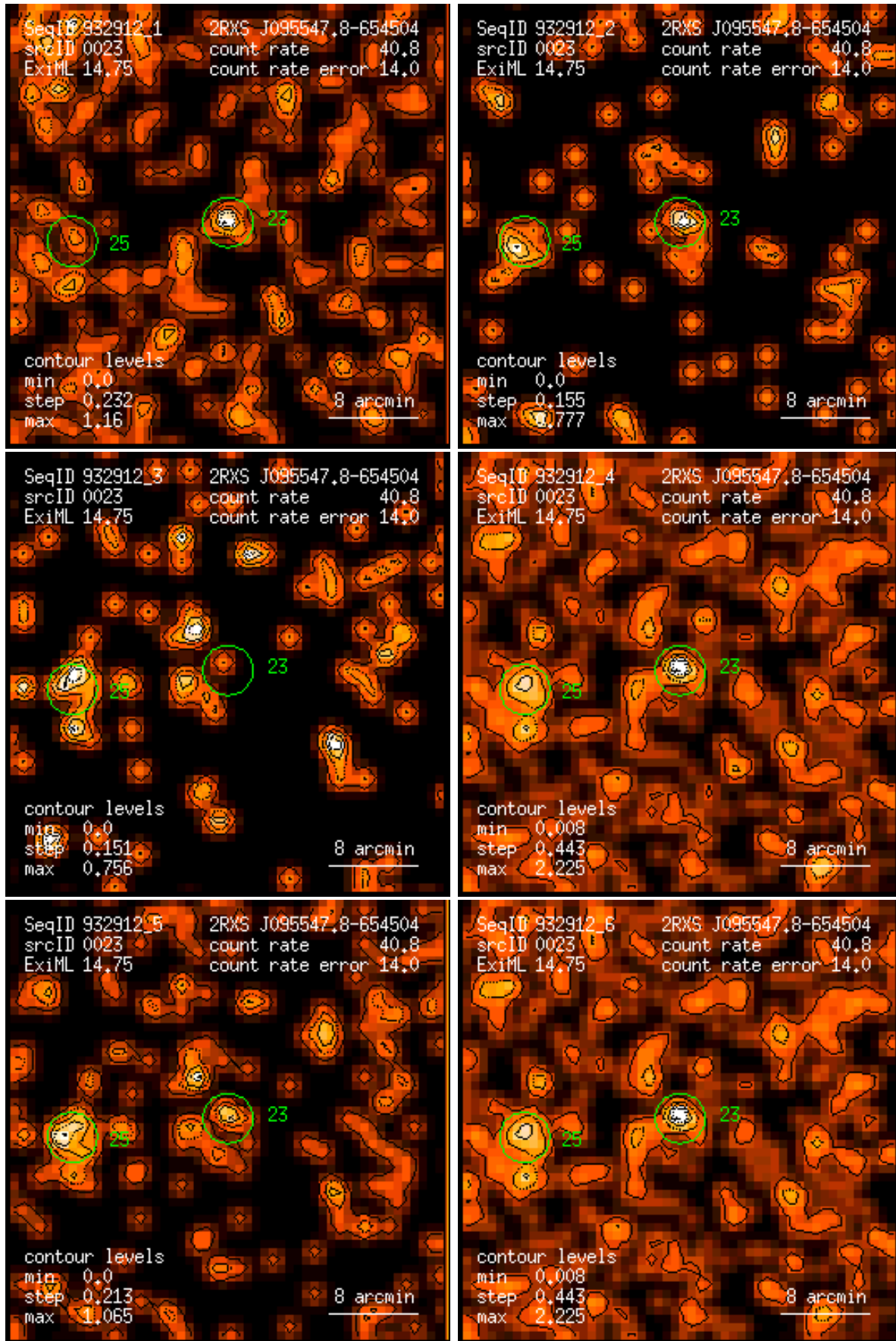
Figure 23: RASS 932912: detection 0023: band rate images, Gaussian filter: (1) PSPC channels 11 – 41, (2) 52 – 90, (3) 91 – 201, (4) 11 – 235, (5) 52 – 201, (6) 11 – 201. Broad band rates in counts/ks. Band rate contour levels in counts/ks/arcmin 2 .
