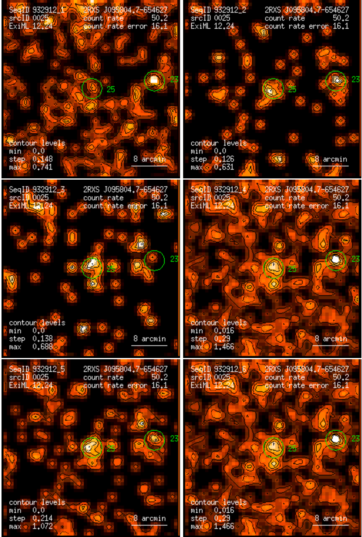
Figure 25: RASS 932912: detection 0025: band rate images, Gaussian filter: (1) PSPC channels 11 – 41, (2) 52 – 90, (3) 91 – 201, (4) 11 – 235, (5) 52 – 201, (6) 11 – 201. Broad band rates in counts/ks. Band rate contour levels in counts/ks/arcmin 2 .
