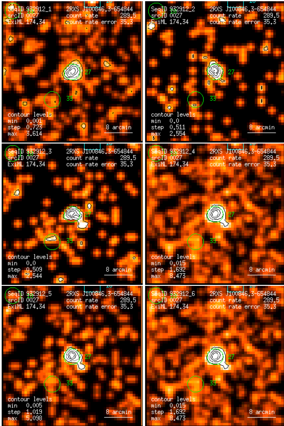
Figure 27: RASS 932912: detection 0027: band rate images, Gaussian filter: (1) PSPC channels 11 – 41, (2) 52 – 90, (3) 91 – 201, (4) 11 – 235, (5) 52 – 201, (6) 11 – 201. Broad band rates in counts/ks. Band rate contour levels in counts/ks/arcmin 2 .
