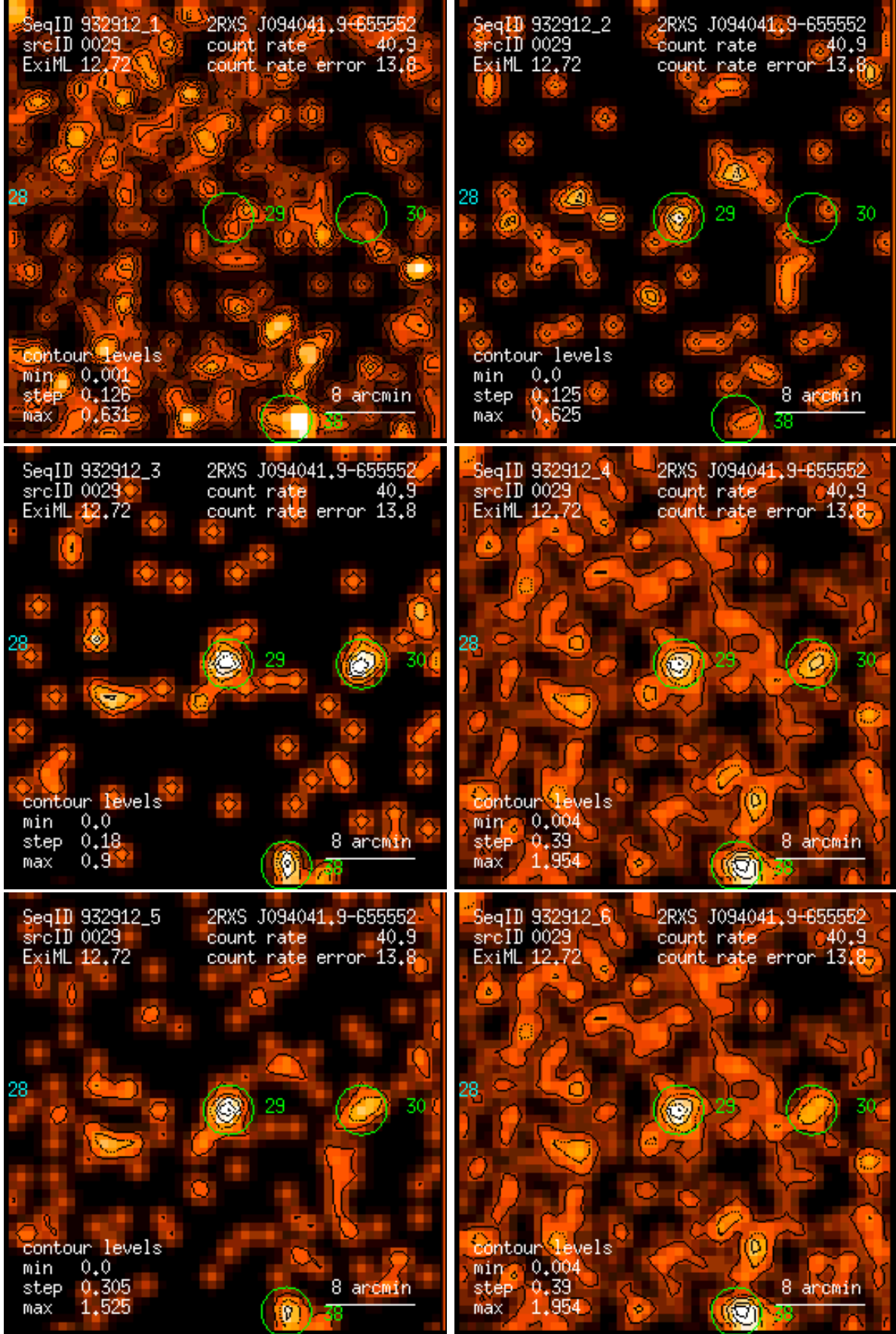
Figure 29: RASS 932912: detection 0029: band rate images, Gaussian filter: (1) PSPC channels 11 – 41, (2) 52 – 90, (3) 91 – 201, (4) 11 – 235, (5) 52 – 201, (6) 11 – 201. Broad band rates in counts/ks. Band rate contour levels in counts/ks/arcmin 2 .
