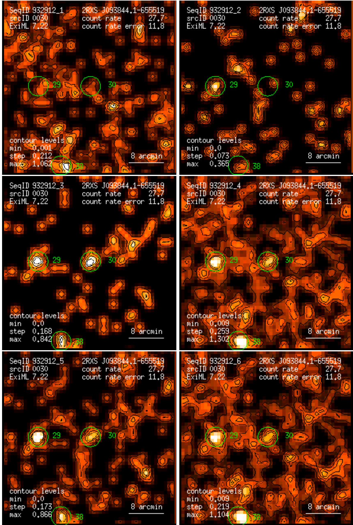
Figure 30: RASS 932912: detection 0030: band rate images, Gaussian filter: (1) PSPC channels 11 – 41, (2) 52 – 90, (3) 91 – 201, (4) 11 – 235, (5) 52 – 201, (6) 11 – 201. Broad band rates in counts/ks. Band rate contour levels in counts/ks/arcmin 2 .
