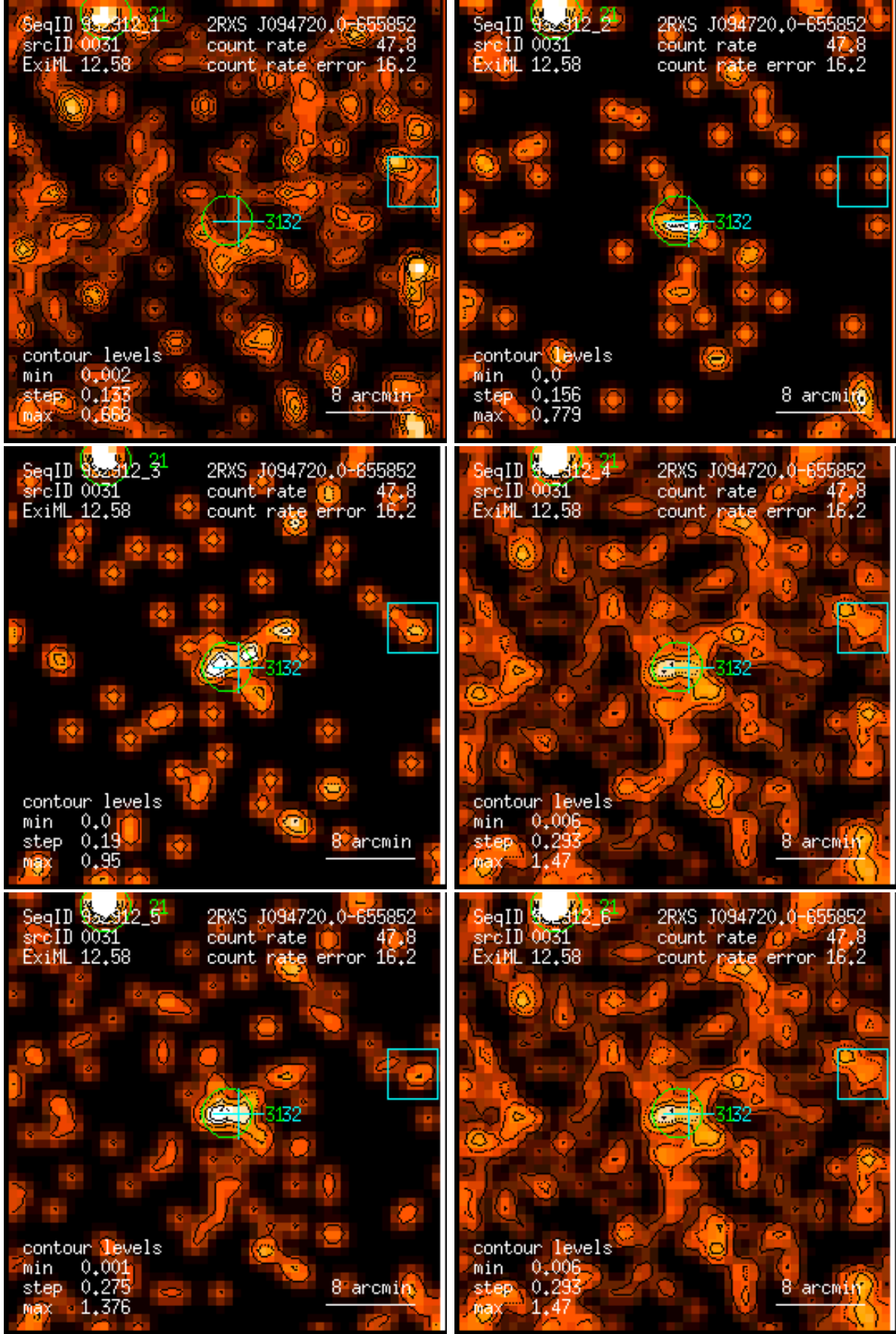
Figure 31: RASS 932912: detection 0031: band rate images, Gaussian filter: (1) PSPC channels 11 – 41, (2) 52 – 90, (3) 91 – 201, (4) 11 – 235, (5) 52 – 201, (6) 11 – 201. Broad band rates in counts/ks. Band rate contour levels in counts/ks/arcmin 2 .
