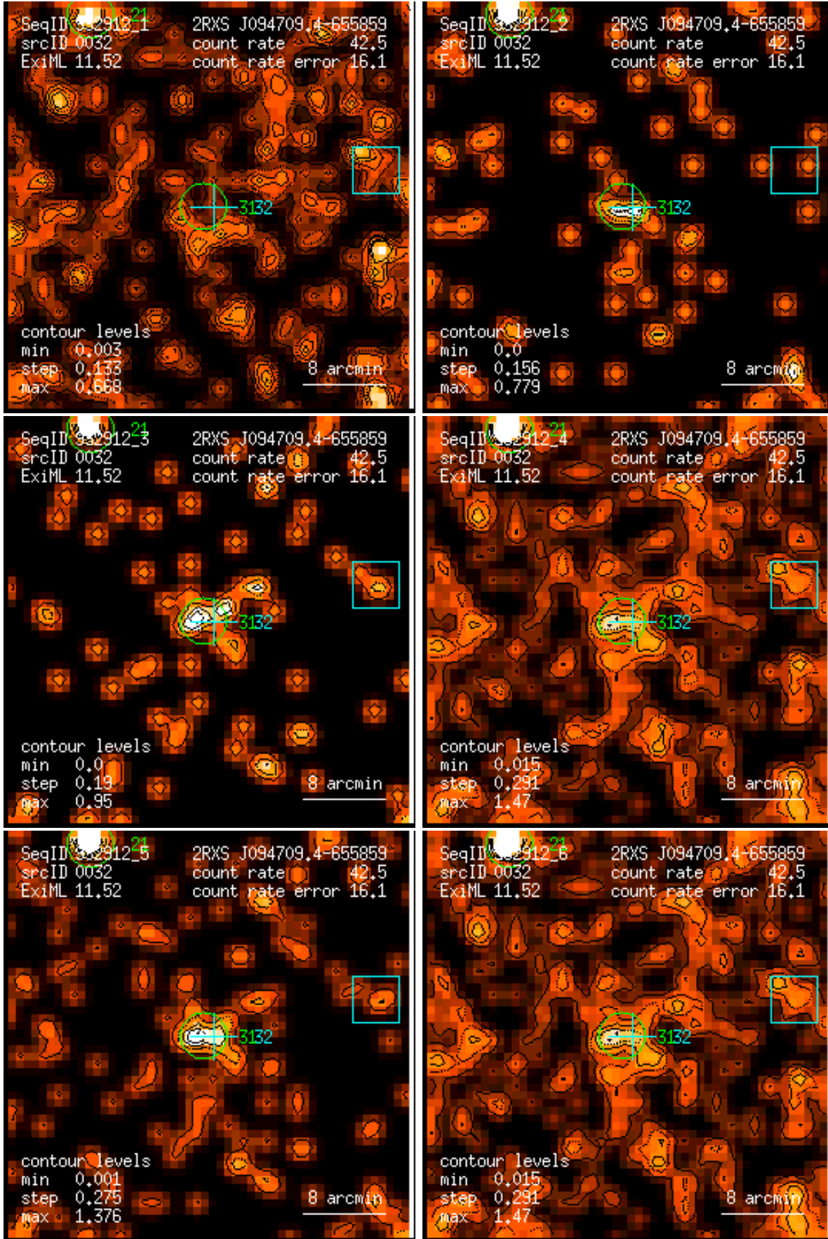
Figure 32: RASS 932912: detection 0032: band rate images, Gaussian filter: (1) PSPC channels 11 – 41, (2) 52 – 90, (3) 91 – 201, (4) 11 – 235, (5) 52 – 201, (6) 11 – 201. Broad band rates in counts/ks. Band rate contour levels in counts/ks/arcmin 2 .
