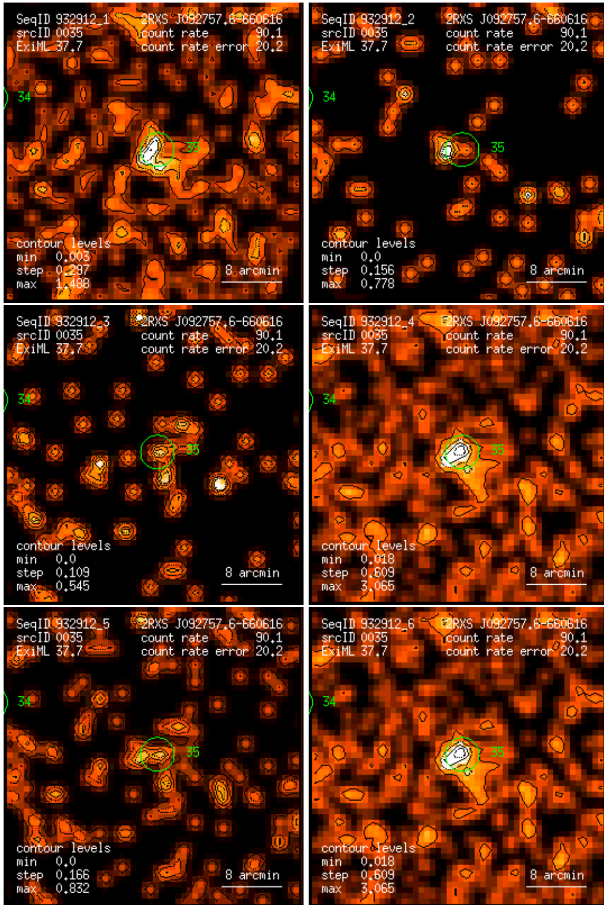
Figure 35: RASS 932912: detection 0035: band rate images, Gaussian filter: (1) PSPC channels 11 – 41, (2) 52 – 90, (3) 91 – 201, (4) 11 – 235, (5) 52 – 201, (6) 11 – 201. Broad band rates in counts/ks. Band rate contour levels in counts/ks/arcmin 2 .
