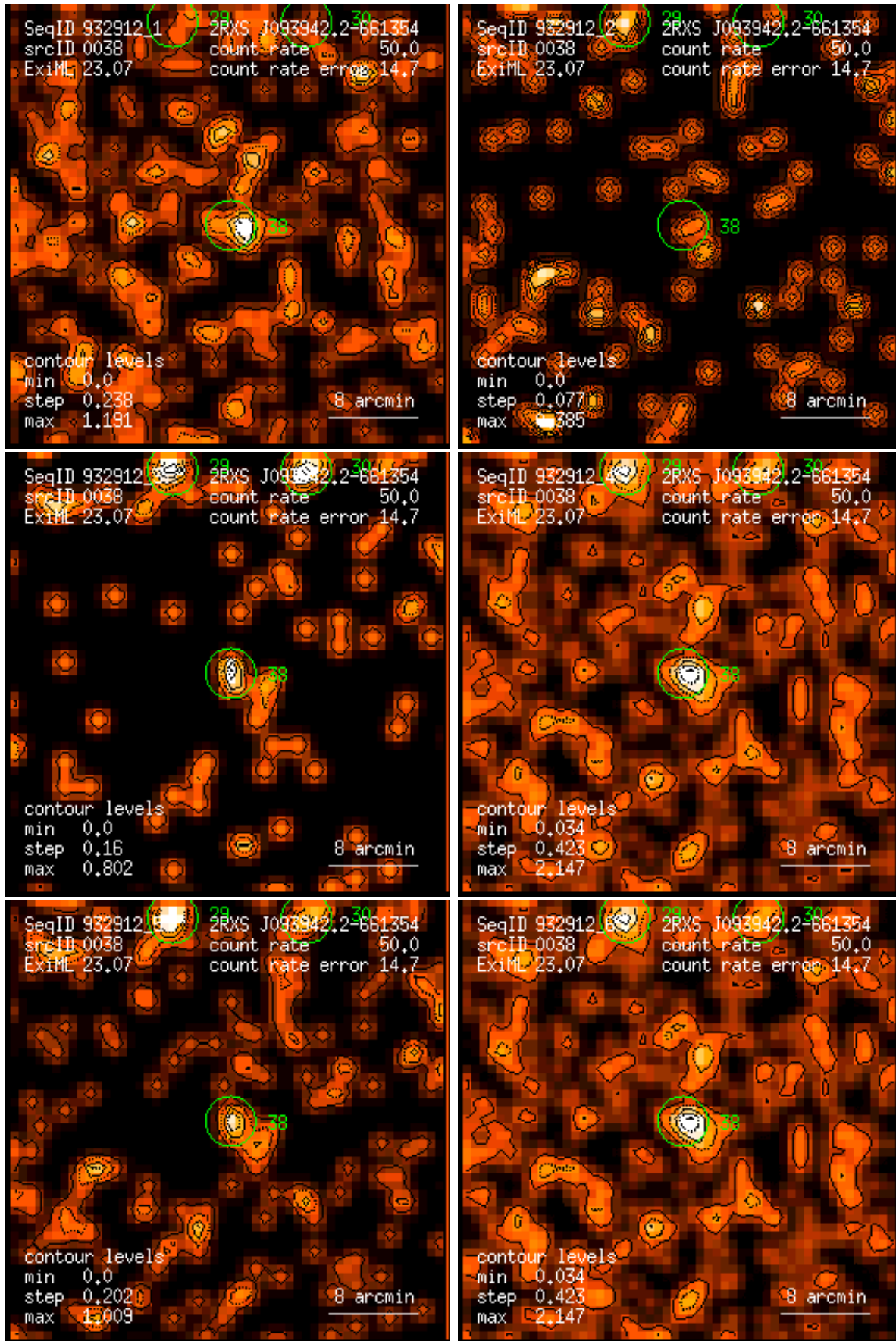
Figure 38: RASS 932912: detection 0038: band rate images, Gaussian filter: (1) PSPC channels 11 – 41, (2) 52 – 90, (3) 91 – 201, (4) 11 – 235, (5) 52 – 201, (6) 11 – 201. Broad band rates in counts/ks. Band rate contour levels in counts/ks/arcmin 2 .
