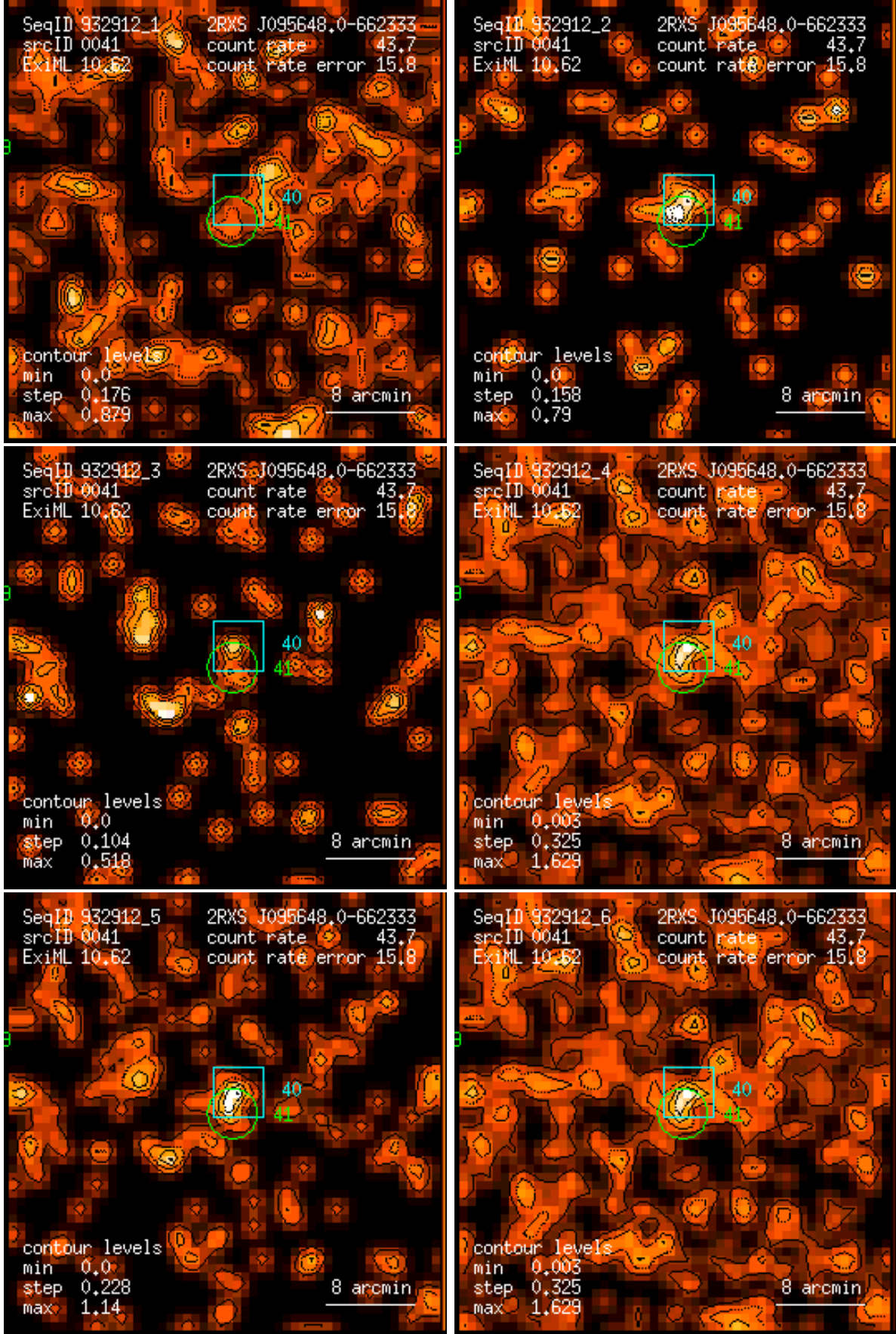
Figure 41: RASS 932912: detection 0041: band rate images, Gaussian filter: (1) PSPC channels 11 – 41, (2) 52 – 90, (3) 91 – 201, (4) 11 – 235, (5) 52 – 201, (6) 11 – 201. Broad band rates in counts/ks. Band rate contour levels in counts/ks/arcmin 2 .
