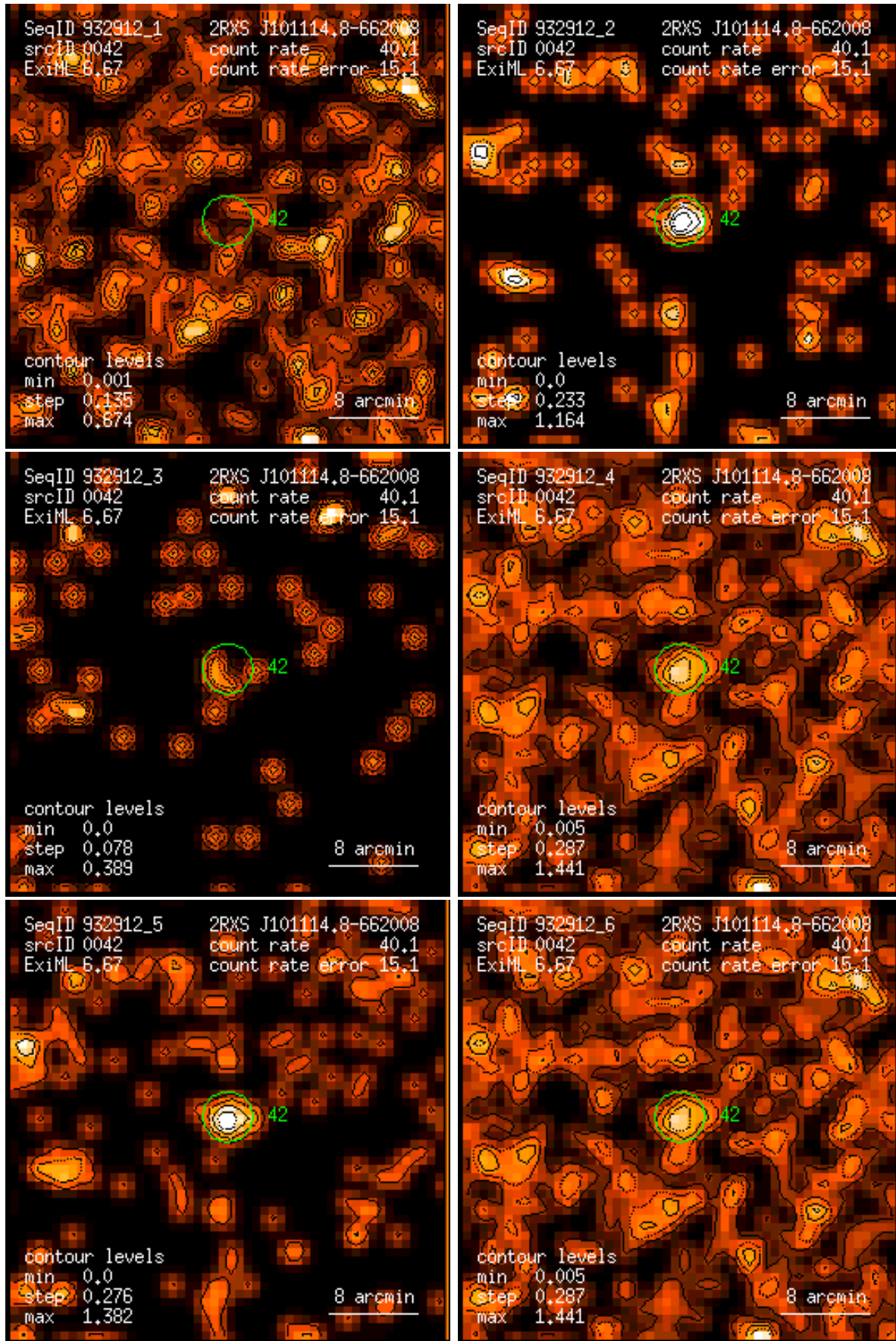
Figure 42: RASS 932912: detection 0042: band rate images, Gaussian filter: (1) PSPC channels 11 – 41, (2) 52 – 90, (3) 91 – 201, (4) 11 – 235, (5) 52 – 201, (6) 11 – 201. Broad band rates in counts/ks. Band rate contour levels in counts/ks/arcmin 2 .
