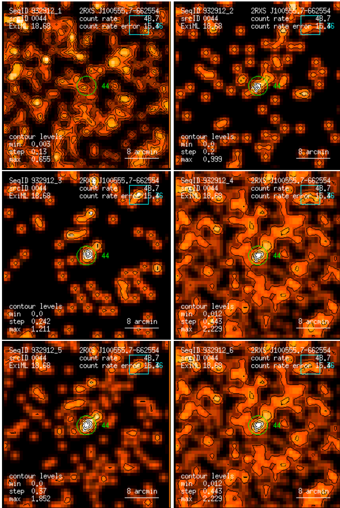
Figure 44: RASS 932912: detection 0044: band rate images, Gaussian filter: (1) PSPC channels 11 – 41, (2) 52 – 90, (3) 91 – 201, (4) 11 – 235, (5) 52 – 201, (6) 11 – 201. Broad band rates in counts/ks. Band rate contour levels in counts/ks/arcmin 2 .
