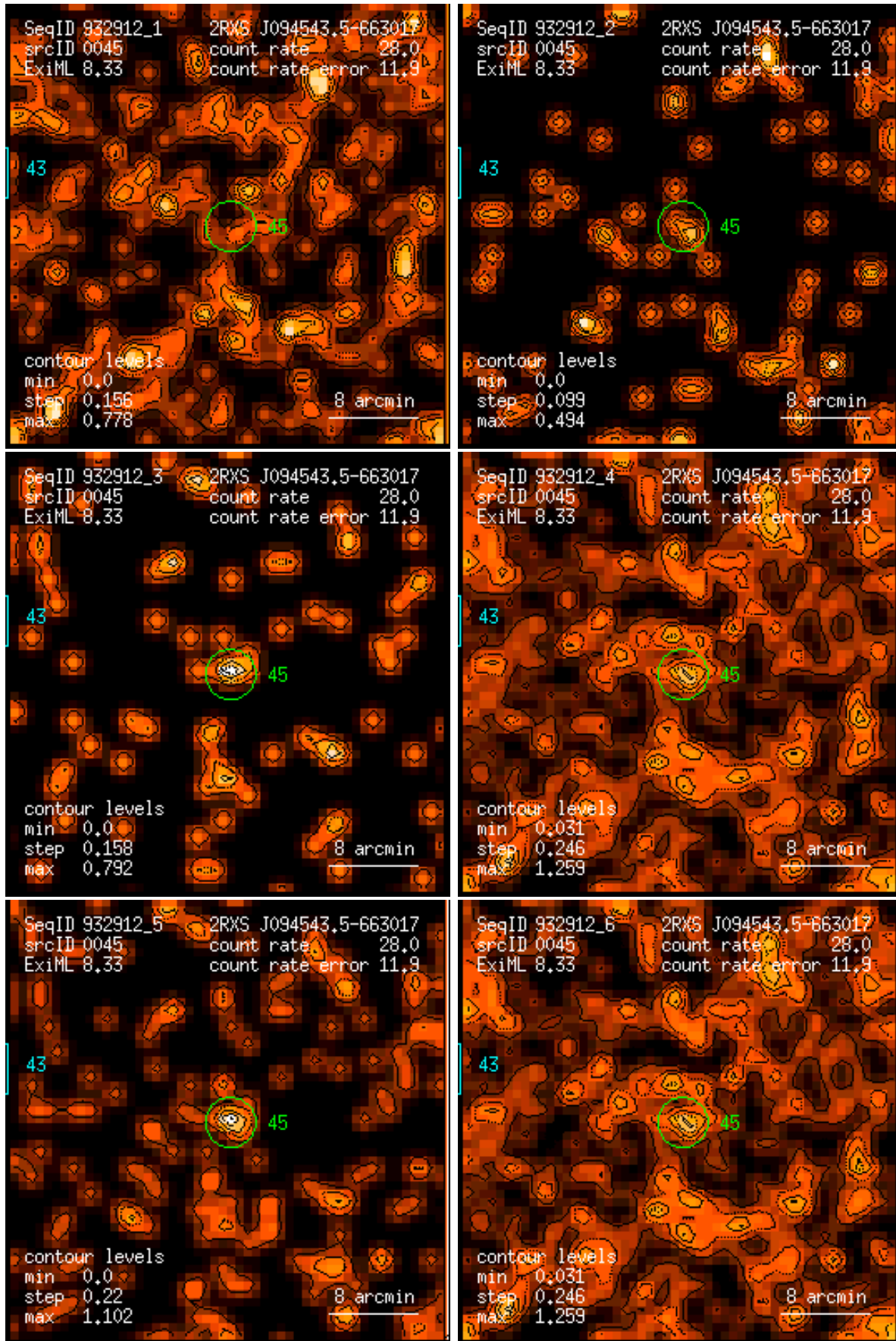
Figure 45: RASS 932912: detection 0045: band rate images, Gaussian filter: (1) PSPC channels 11 – 41, (2) 52 – 90, (3) 91 – 201, (4) 11 – 235, (5) 52 – 201, (6) 11 – 201. Broad band rates in counts/ks. Band rate contour levels in counts/ks/arcmin 2 .
