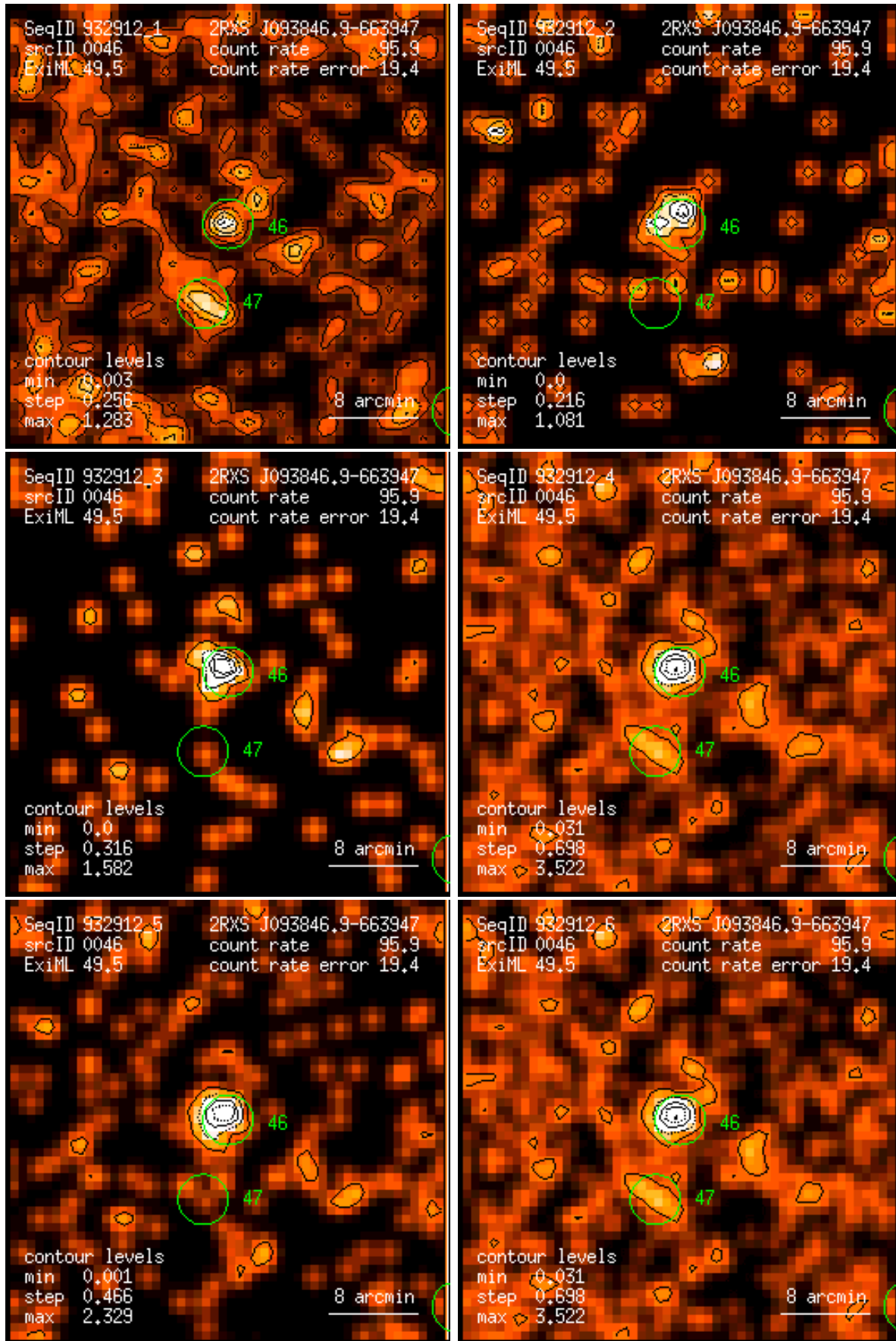
Figure 46: RASS 932912: detection 0046: band rate images, Gaussian filter: (1) PSPC channels 11 – 41, (2) 52 – 90, (3) 91 – 201, (4) 11 – 235, (5) 52 – 201, (6) 11 – 201. Broad band rates in counts/ks. Band rate contour levels in counts/ks/arcmin 2 .
