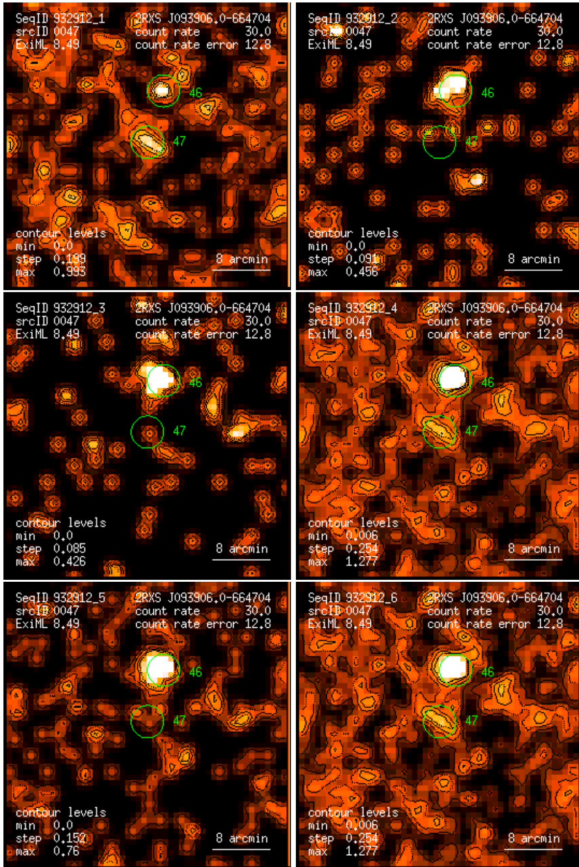
Figure 47: RASS 932912: detection 0047: band rate images, Gaussian filter: (1) PSPC channels 11 – 41, (2) 52 – 90, (3) 91 – 201, (4) 11 – 235, (5) 52 – 201, (6) 11 – 201. Broad band rates in counts/ks. Band rate contour levels in counts/ks/arcmin 2 .
