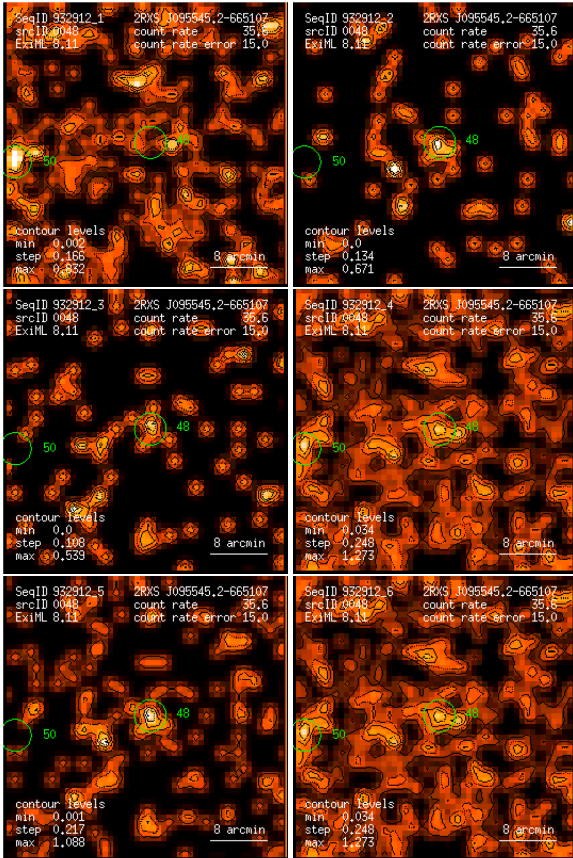
Figure 48: RASS 932912: detection 0048: band rate images, Gaussian filter: (1) PSPC channels 11 – 41, (2) 52 – 90, (3) 91 – 201, (4) 11 – 235, (5) 52 – 201, (6) 11 – 201. Broad band rates in counts/ks. Band rate contour levels in counts/ks/arcmin 2 .
