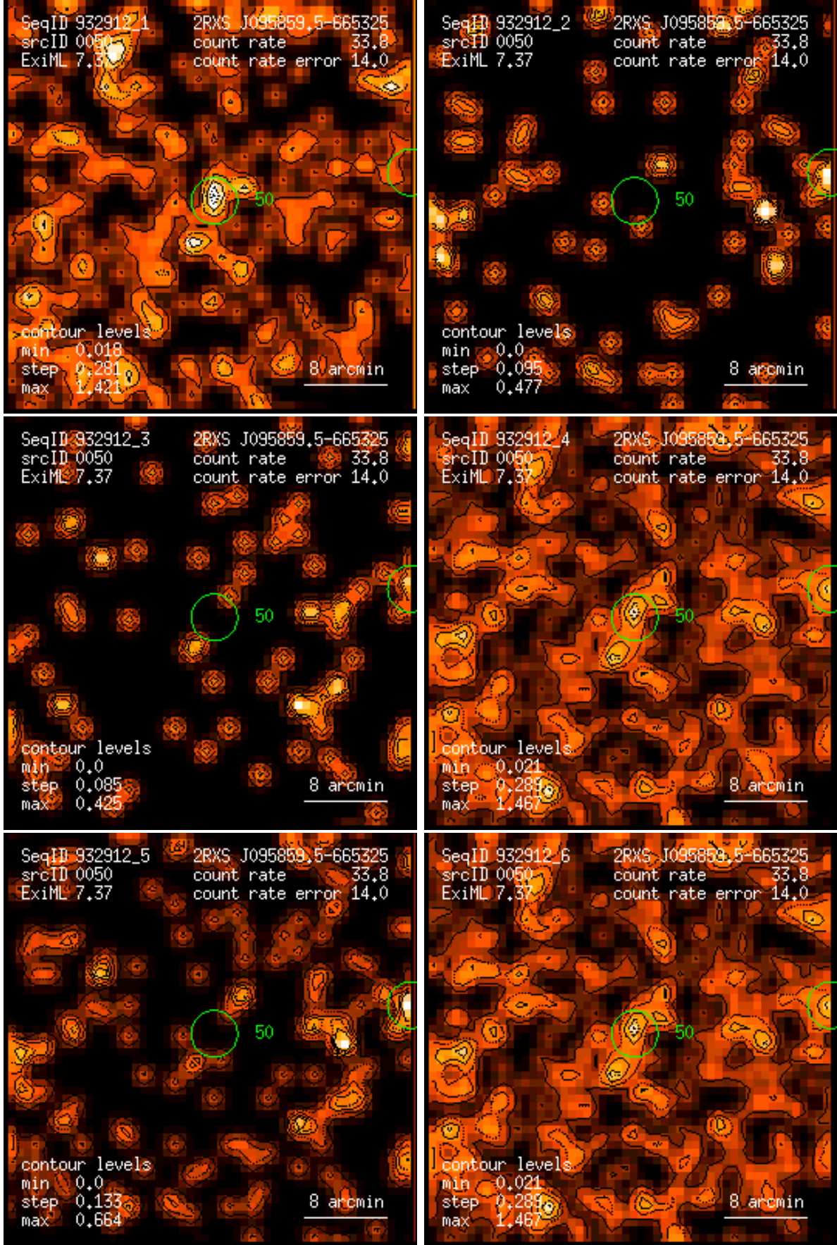
Figure 50: RASS 932912: detection 0050: band rate images, Gaussian filter: (1) PSPC channels 11 – 41, (2) 52 – 90, (3) 91 – 201, (4) 11 – 235, (5) 52 – 201, (6) 11 – 201. Broad band rates in counts/ks. Band rate contour levels in counts/ks/arcmin 2 .
