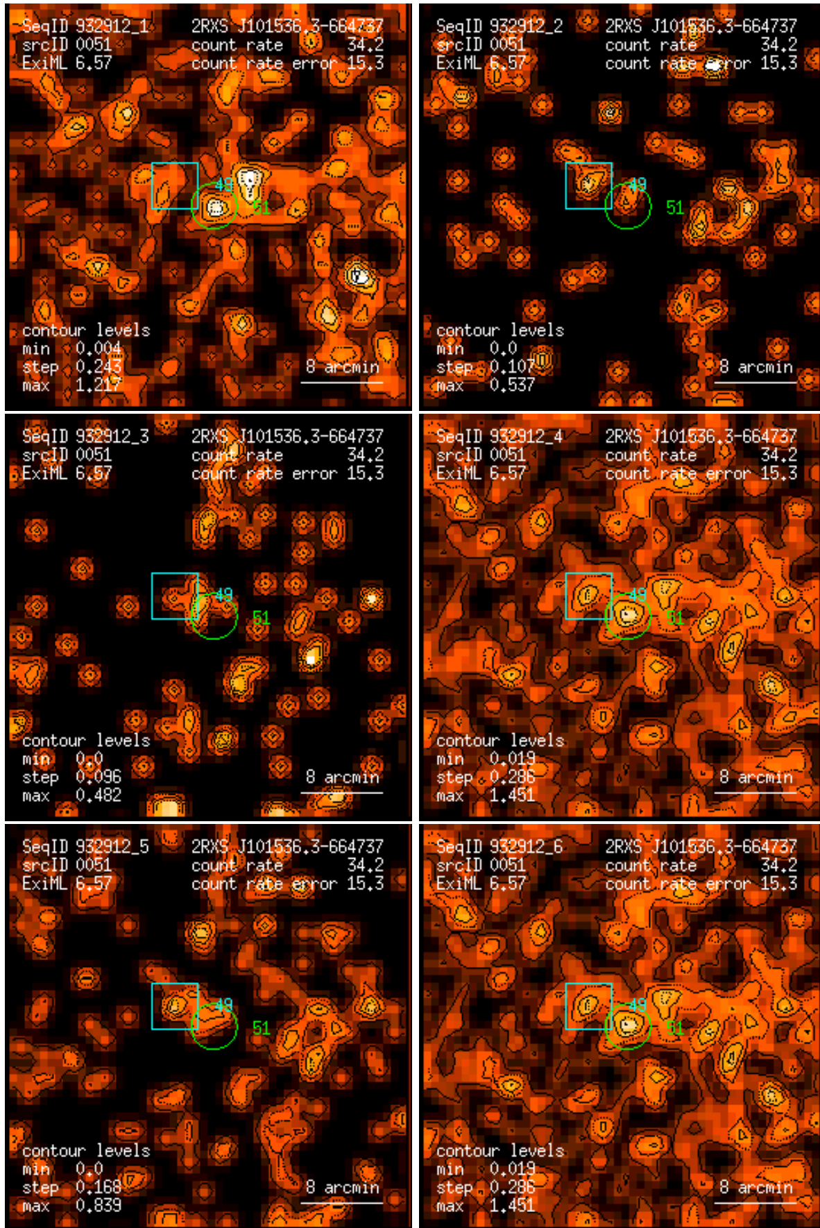
Figure 51: RASS 932912: detection 0051: band rate images, Gaussian filter: (1) PSPC channels 11 – 41, (2) 52 – 90, (3) 91 – 201, (4) 11 – 235, (5) 52 – 201, (6) 11 – 201. Broad band rates in counts/ks. Band rate contour levels in counts/ks/arcmin 2 .
