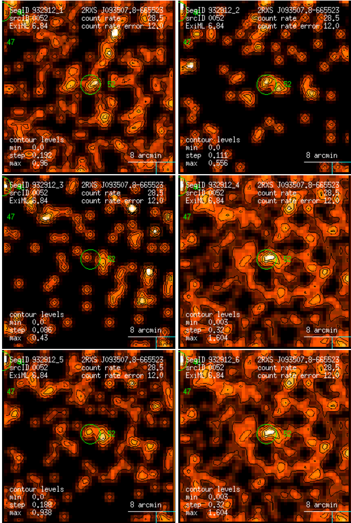
Figure 52: RASS 932912: detection 0052: band rate images, Gaussian filter: (1) PSPC channels 11 – 41, (2) 52 – 90, (3) 91 – 201, (4) 11 – 235, (5) 52 – 201, (6) 11 – 201. Broad band rates in counts/ks. Band rate contour levels in counts/ks/arcmin 2 .
