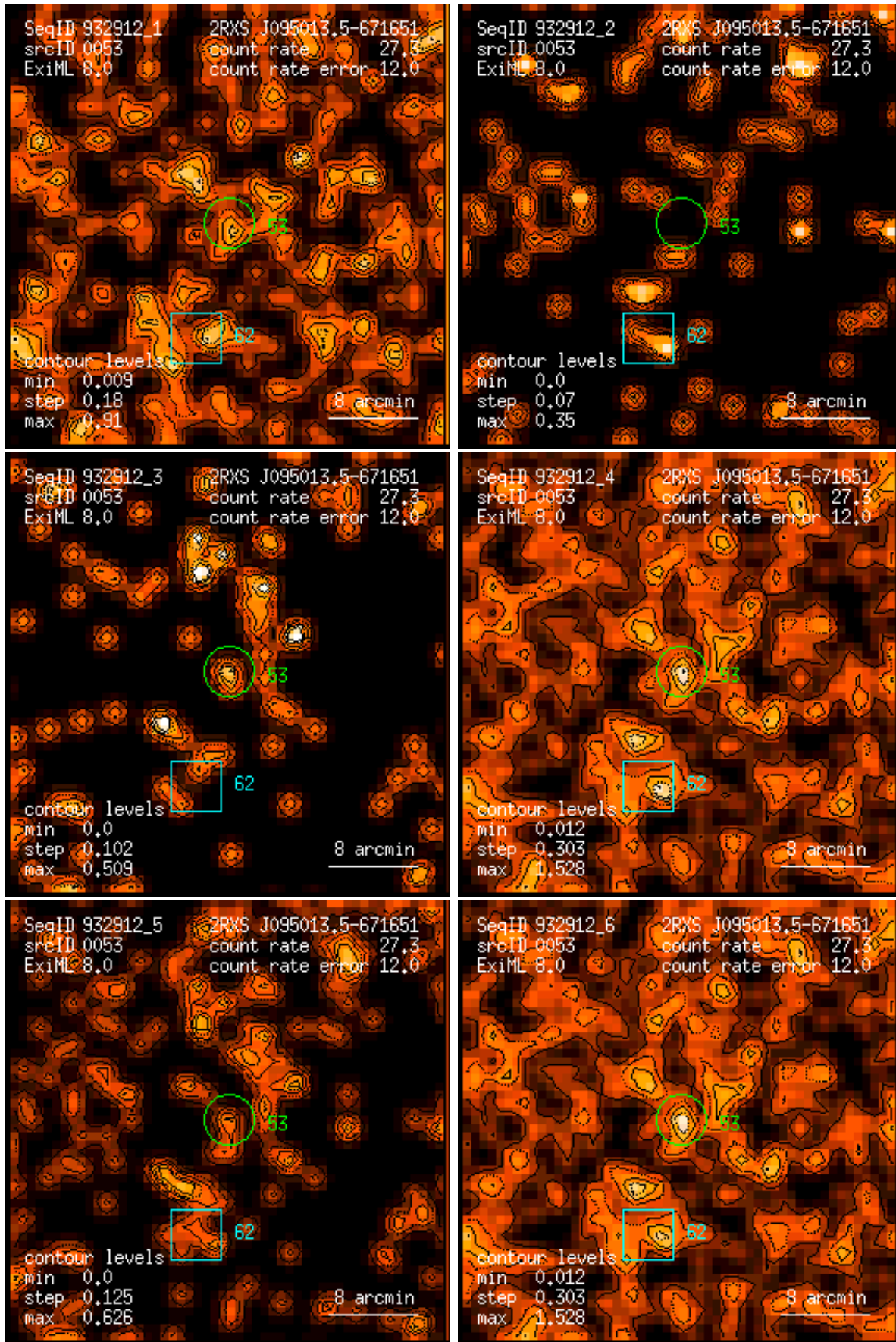
Figure 53: RASS 932912: detection 0053: band rate images, Gaussian filter: (1) PSPC channels 11 – 41, (2) 52 – 90, (3) 91 – 201, (4) 11 – 235, (5) 52 – 201, (6) 11 – 201. Broad band rates in counts/ks. Band rate contour levels in counts/ks/arcmin 2 .
