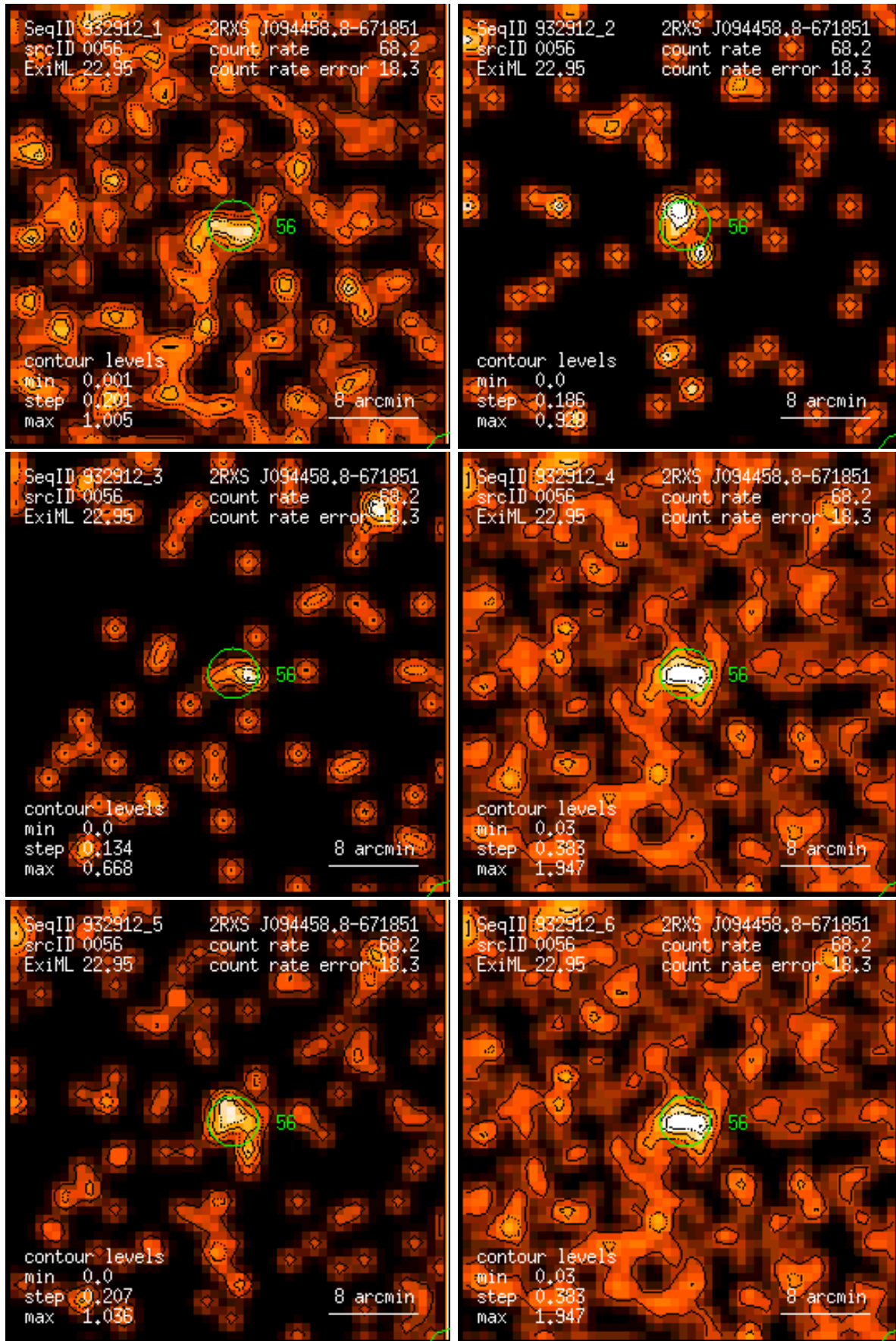
Figure 56: RASS 932912: detection 0056: band rate images, Gaussian filter: (1) PSPC channels 11 – 41, (2) 52 – 90, (3) 91 – 201, (4) 11 – 235, (5) 52 – 201, (6) 11 – 201. Broad band rates in counts/ks. Band rate contour levels in counts/ks/arcmin 2 .
