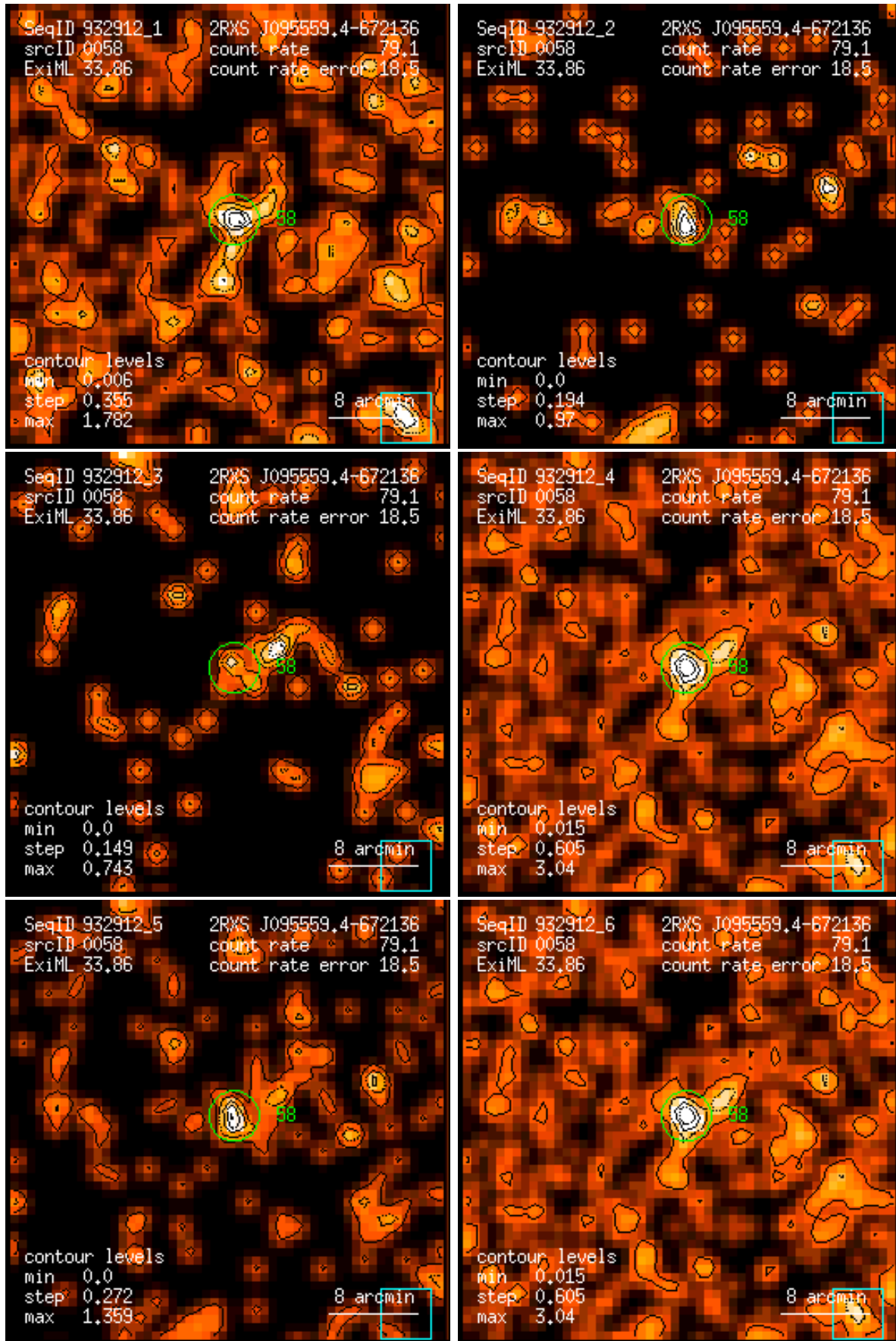
Figure 58: RASS 932912: detection 0058: band rate images, Gaussian filter: (1) PSPC channels 11 – 41, (2) 52 – 90, (3) 91 – 201, (4) 11 – 235, (5) 52 – 201, (6) 11 – 201. Broad band rates in counts/ks. Band rate contour levels in counts/ks/arcmin 2 .
