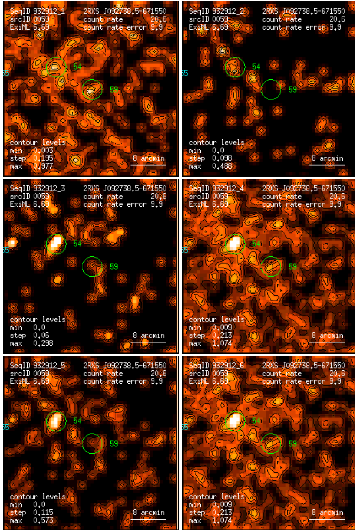
Figure 59: RASS 932912: detection 0059: band rate images, Gaussian filter: (1) PSPC channels 11 – 41, (2) 52 – 90, (3) 91 – 201, (4) 11 – 235, (5) 52 – 201, (6) 11 – 201. Broad band rates in counts/ks. Band rate contour levels in counts/ks/arcmin 2 .
