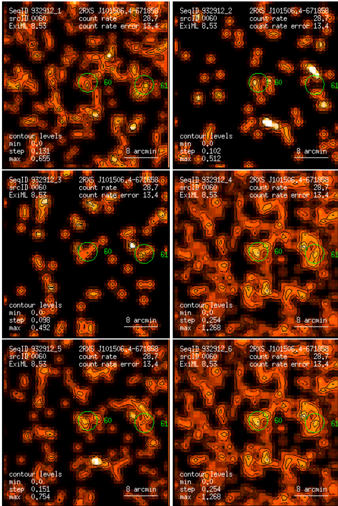
Figure 60: RASS 932912: detection 0060: band rate images, Gaussian filter: (1) PSPC channels 11 – 41, (2) 52 – 90, (3) 91 – 201, (4) 11 – 235, (5) 52 – 201, (6) 11 – 201. Broad band rates in counts/ks. Band rate contour levels in counts/ks/arcmin 2 .
