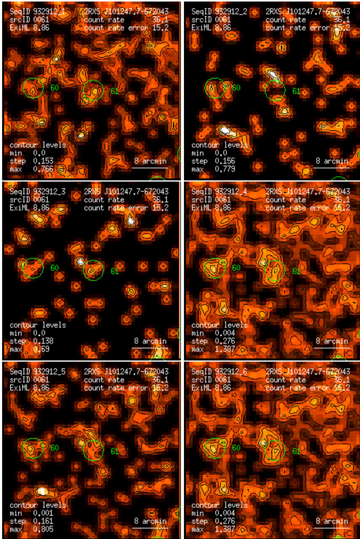
Figure 61: RASS 932912: detection 0061: band rate images, Gaussian filter: (1) PSPC channels 11 – 41, (2) 52 – 90, (3) 91 – 201, (4) 11 – 235, (5) 52 – 201, (6) 11 – 201. Broad band rates in counts/ks. Band rate contour levels in counts/ks/arcmin 2 .
