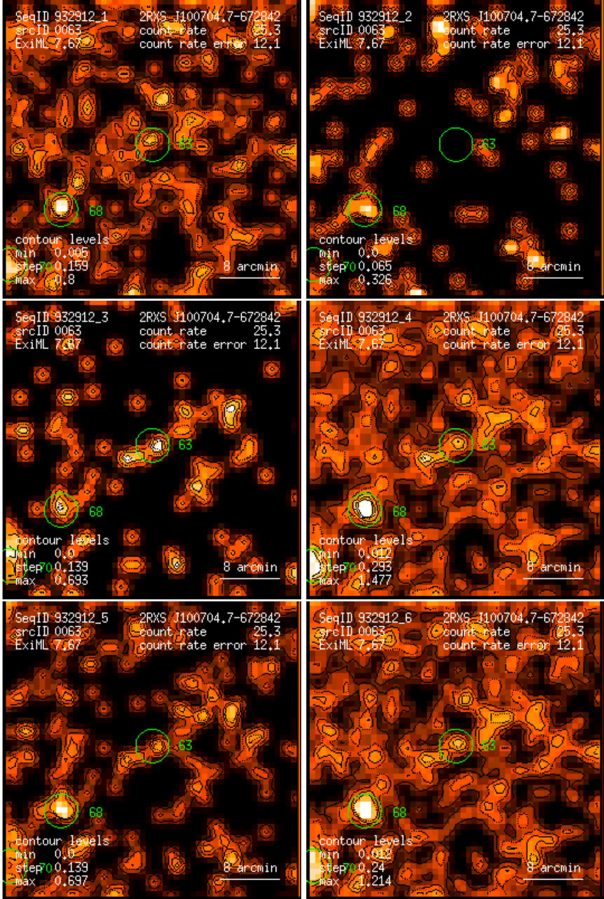
Figure 63: RASS 932912: detection 0063: band rate images, Gaussian filter: (1) PSPC channels 11 – 41, (2) 52 – 90, (3) 91 – 201, (4) 11 – 235, (5) 52 – 201, (6) 11 – 201. Broad band rates in counts/ks. Band rate contour levels in counts/ks/arcmin 2 .
