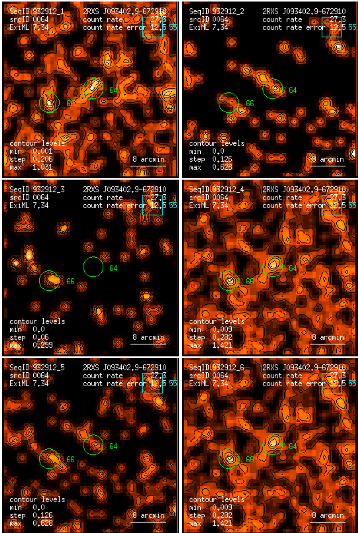
Figure 64: RASS 932912: detection 0064: band rate images, Gaussian filter: (1) PSPC channels 11 – 41, (2) 52 – 90, (3) 91 – 201, (4) 11 – 235, (5) 52 – 201, (6) 11 – 201. Broad band rates in counts/ks. Band rate contour levels in counts/ks/arcmin 2 .
