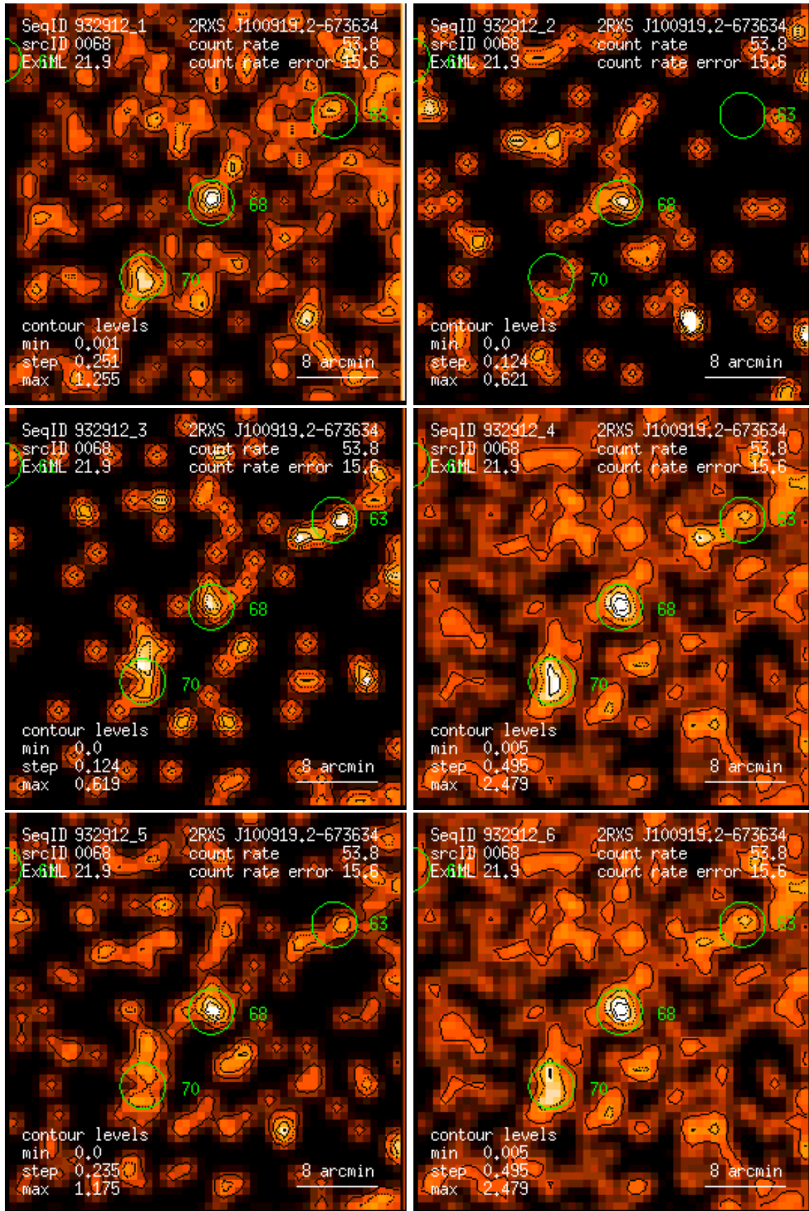
Figure 68: RASS 932912: detection 0068: band rate images, Gaussian filter: (1) PSPC channels 11 – 41, (2) 52 – 90, (3) 91 – 201, (4) 11 – 235, (5) 52 – 201, (6) 11 – 201. Broad band rates in counts/ks. Band rate contour levels in counts/ks/arcmin 2 .
