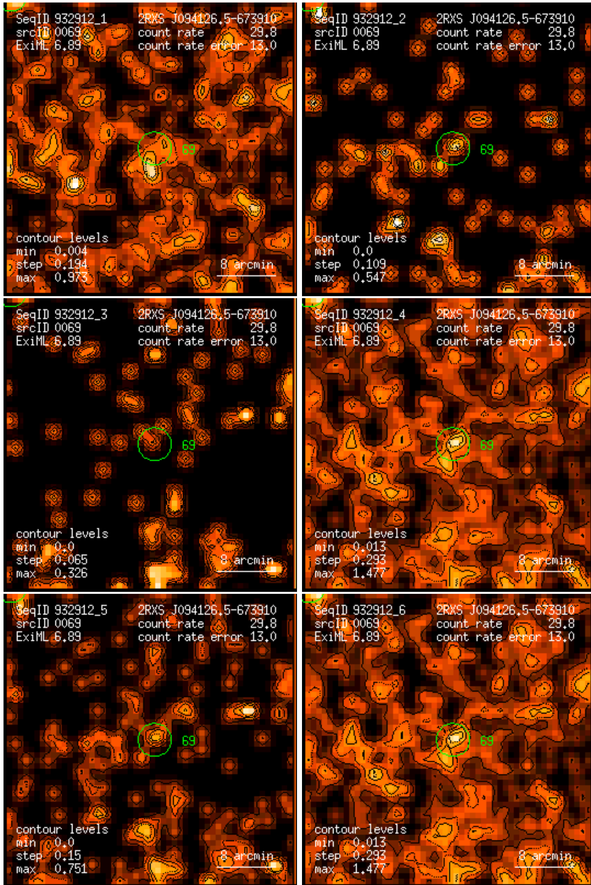
Figure 69: RASS 932912: detection 0069: band rate images, Gaussian filter: (1) PSPC channels 11 – 41, (2) 52 – 90, (3) 91 – 201, (4) 11 – 235, (5) 52 – 201, (6) 11 – 201. Broad band rates in counts/ks. Band rate contour levels in counts/ks/arcmin 2 .
