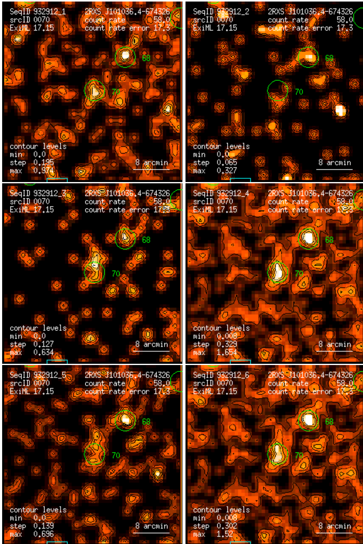
Figure 70: RASS 932912: detection 0070: band rate images, Gaussian filter: (1) PSPC channels 11 – 41, (2) 52 – 90, (3) 91 – 201, (4) 11 – 235, (5) 52 – 201, (6) 11 – 201. Broad band rates in counts/ks. Band rate contour levels in counts/ks/arcmin 2 .
