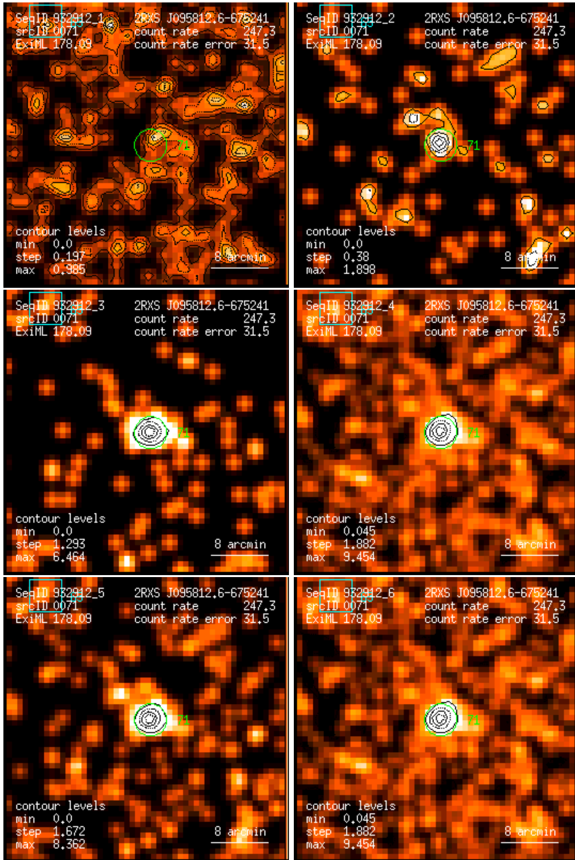
Figure 71: RASS 932912: detection 0071: band rate images, Gaussian filter: (1) PSPC channels 11 – 41, (2) 52 – 90, (3) 91 – 201, (4) 11 – 235, (5) 52 – 201, (6) 11 – 201. Broad band rates in counts/ks. Band rate contour levels in counts/ks/arcmin 2 .
