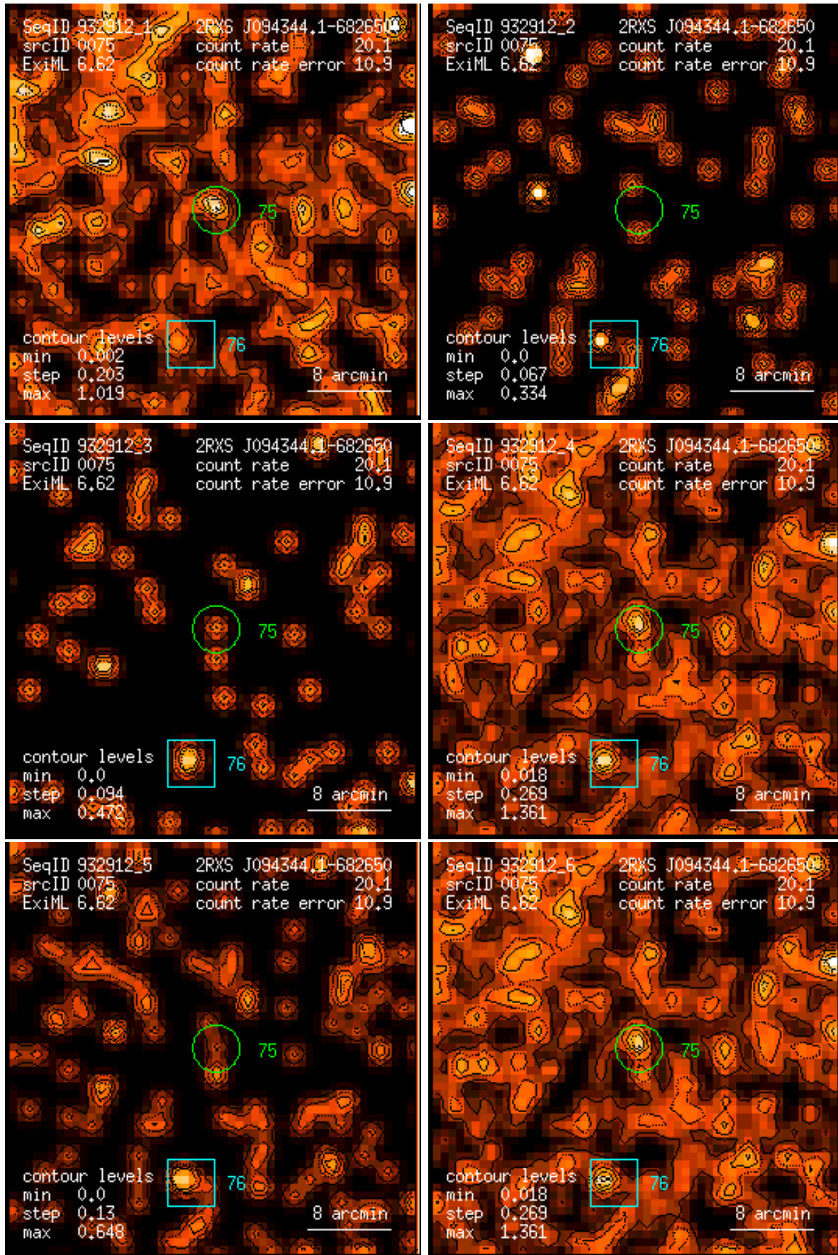
Figure 75: RASS 932912: detection 0075: band rate images, Gaussian filter: (1) PSPC channels 11 – 41, (2) 52 – 90, (3) 91 – 201, (4) 11 – 235, (5) 52 – 201, (6) 11 – 201. Broad band rates in counts/ks. Band rate contour levels in counts/ks/arcmin 2 .
