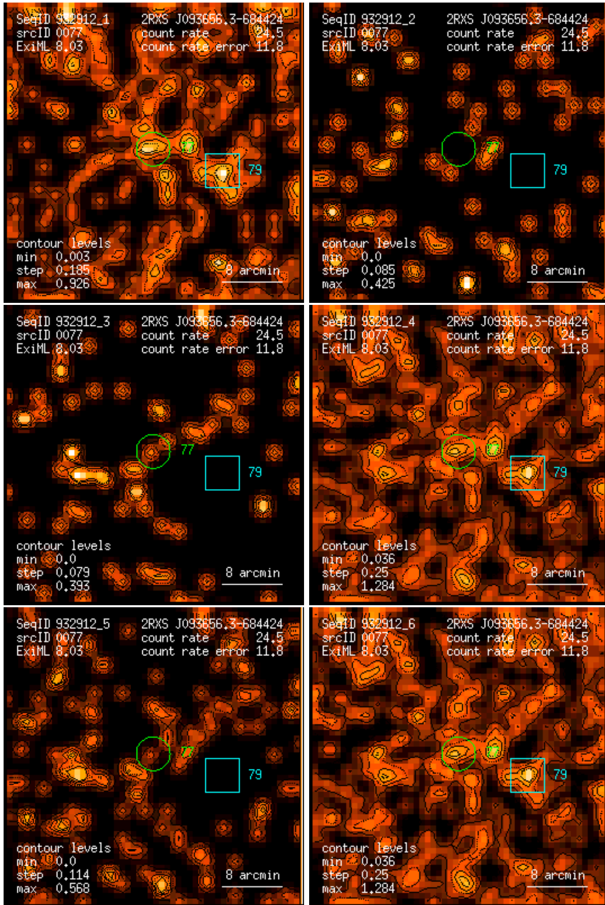
Figure 77: RASS 932912: detection 0077: band rate images, Gaussian filter: (1) PSPC channels 11 – 41, (2) 52 – 90, (3) 91 – 201, (4) 11 – 235, (5) 52 – 201, (6) 11 – 201. Broad band rates in counts/ks. Band rate contour levels in counts/ks/arcmin 2 .
