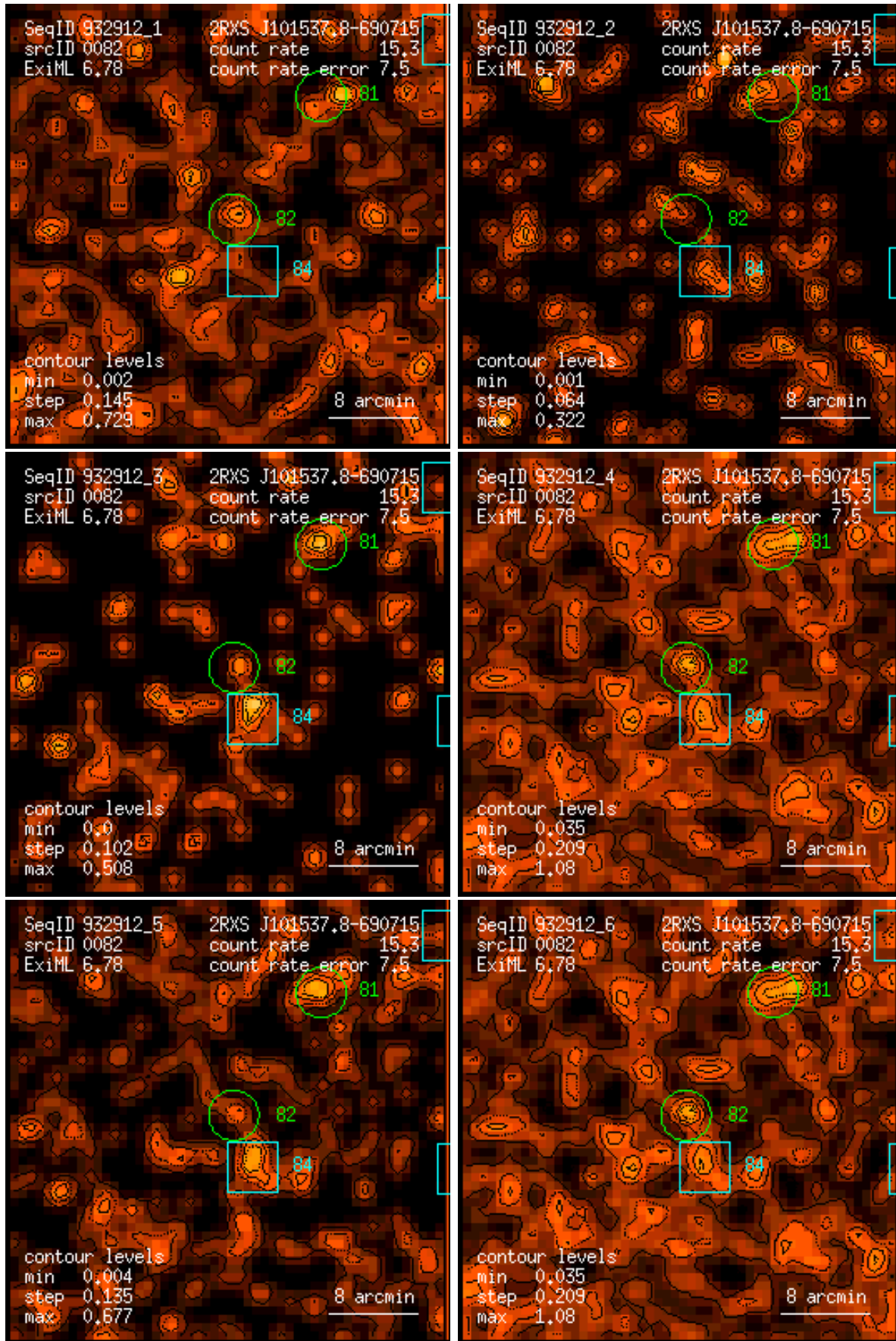
Figure 82: RASS 932912: detection 0082: band rate images, Gaussian filter: (1) PSPC channels 11 – 41, (2) 52 – 90, (3) 91 – 201, (4) 11 – 235, (5) 52 – 201, (6) 11 – 201. Broad band rates in counts/ks. Band rate contour levels in counts/ks/arcmin 2 .
