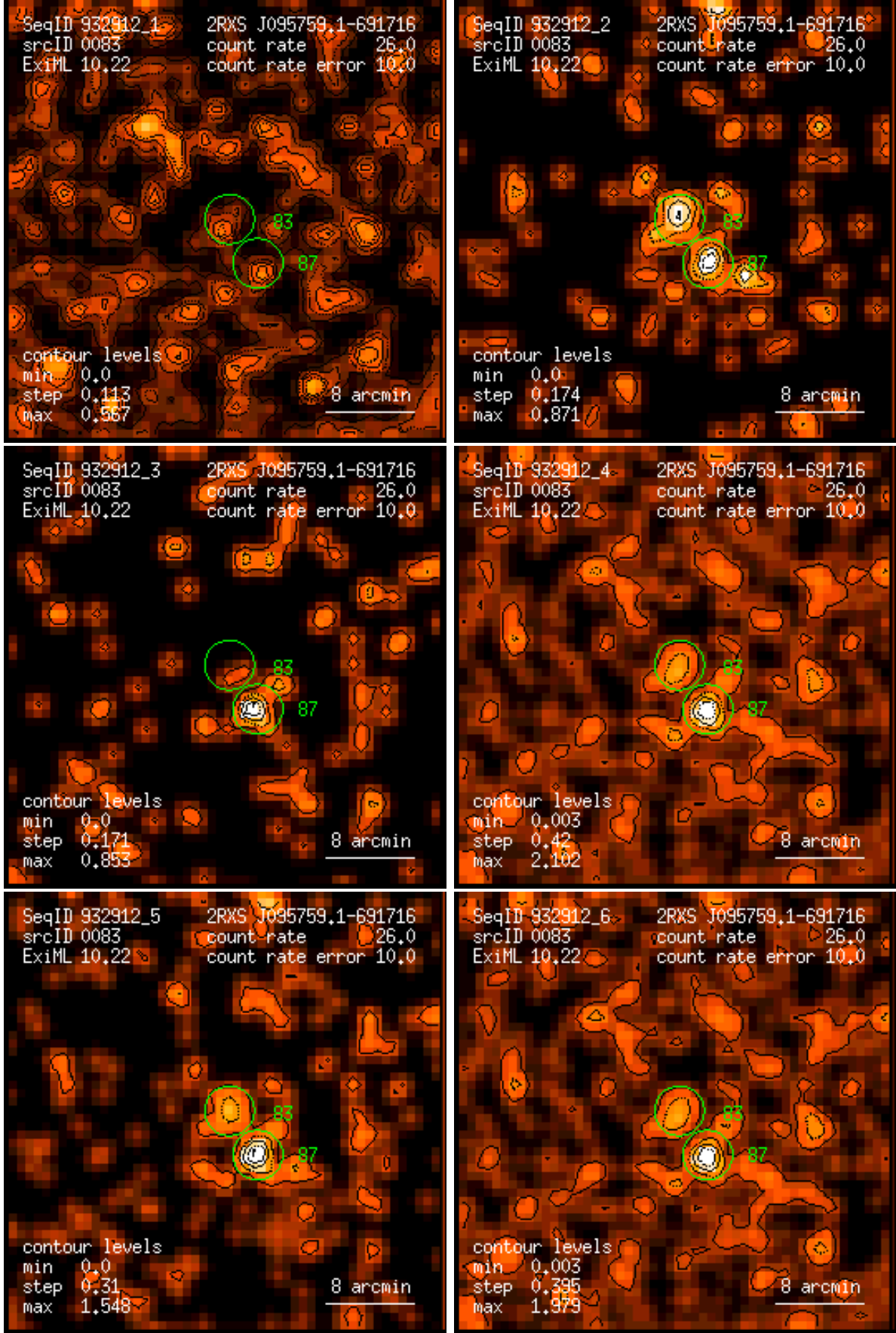
Figure 83: RASS 932912: detection 0083: band rate images, Gaussian filter: (1) PSPC channels 11 – 41, (2) 52 – 90, (3) 91 – 201, (4) 11 – 235, (5) 52 – 201, (6) 11 – 201. Broad band rates in counts/ks. Band rate contour levels in counts/ks/arcmin 2 .
