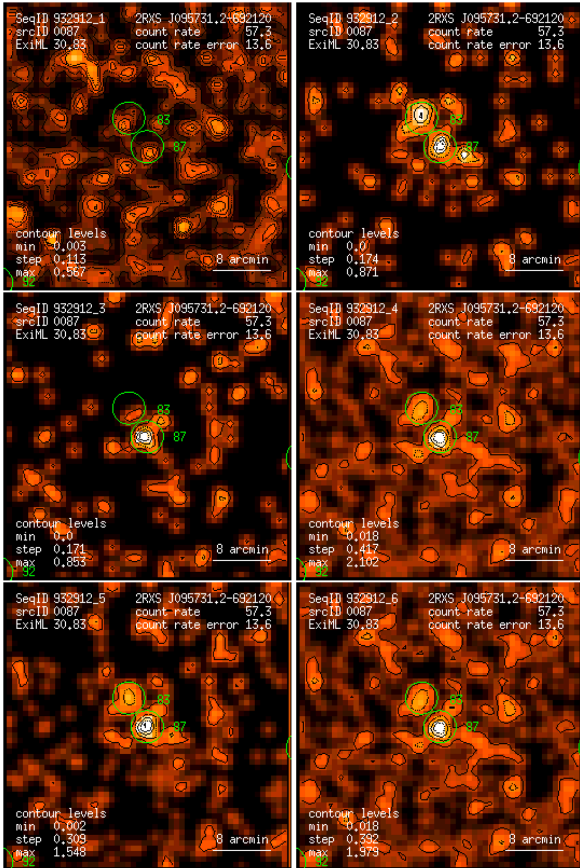
Figure 87: RASS 932912: detection 0087: band rate images, Gaussian filter: (1) PSPC channels 11 – 41, (2) 52 – 90, (3) 91 – 201, (4) 11 – 235, (5) 52 – 201, (6) 11 – 201. Broad band rates in counts/ks. Band rate contour levels in counts/ks/arcmin 2 .
