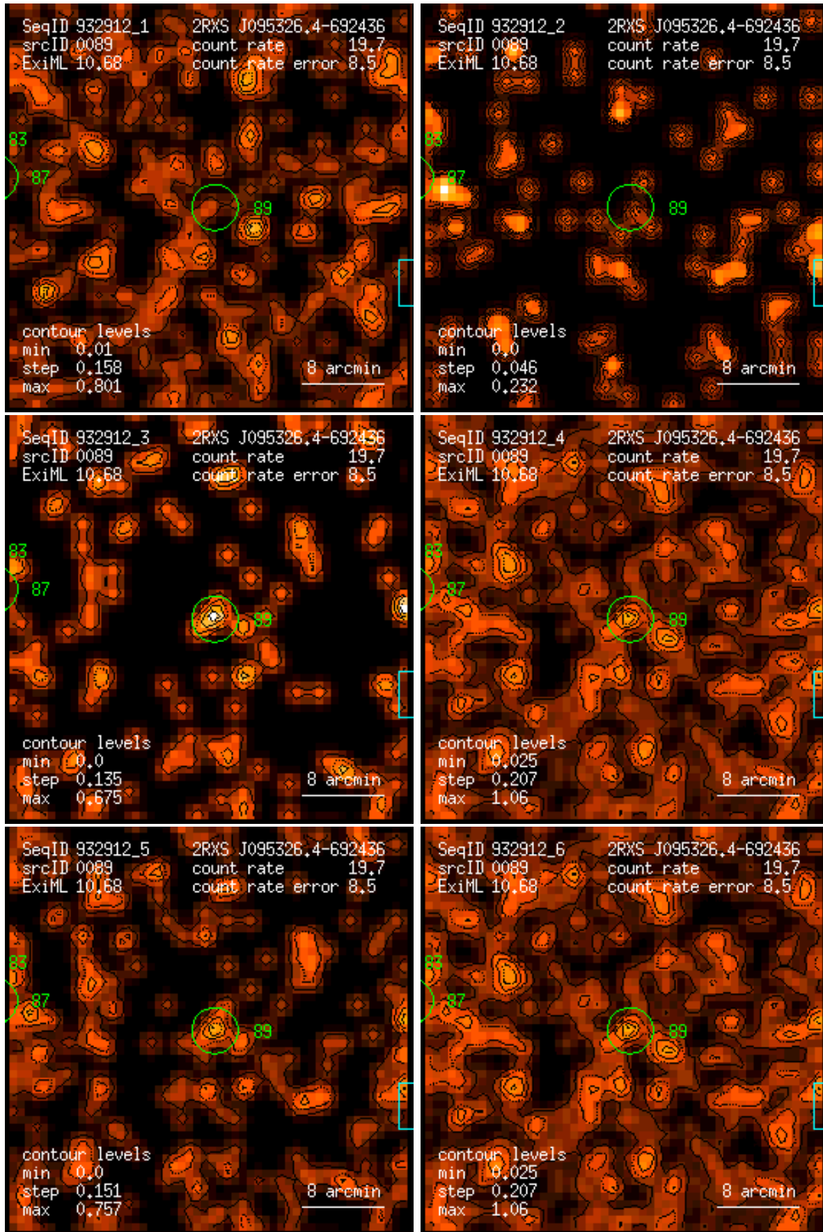
Figure 89: RASS 932912: detection 0089: band rate images, Gaussian filter: (1) PSPC channels 11 – 41, (2) 52 – 90, (3) 91 – 201, (4) 11 – 235, (5) 52 – 201, (6) 11 – 201. Broad band rates in counts/ks. Band rate contour levels in counts/ks/arcmin 2 .
