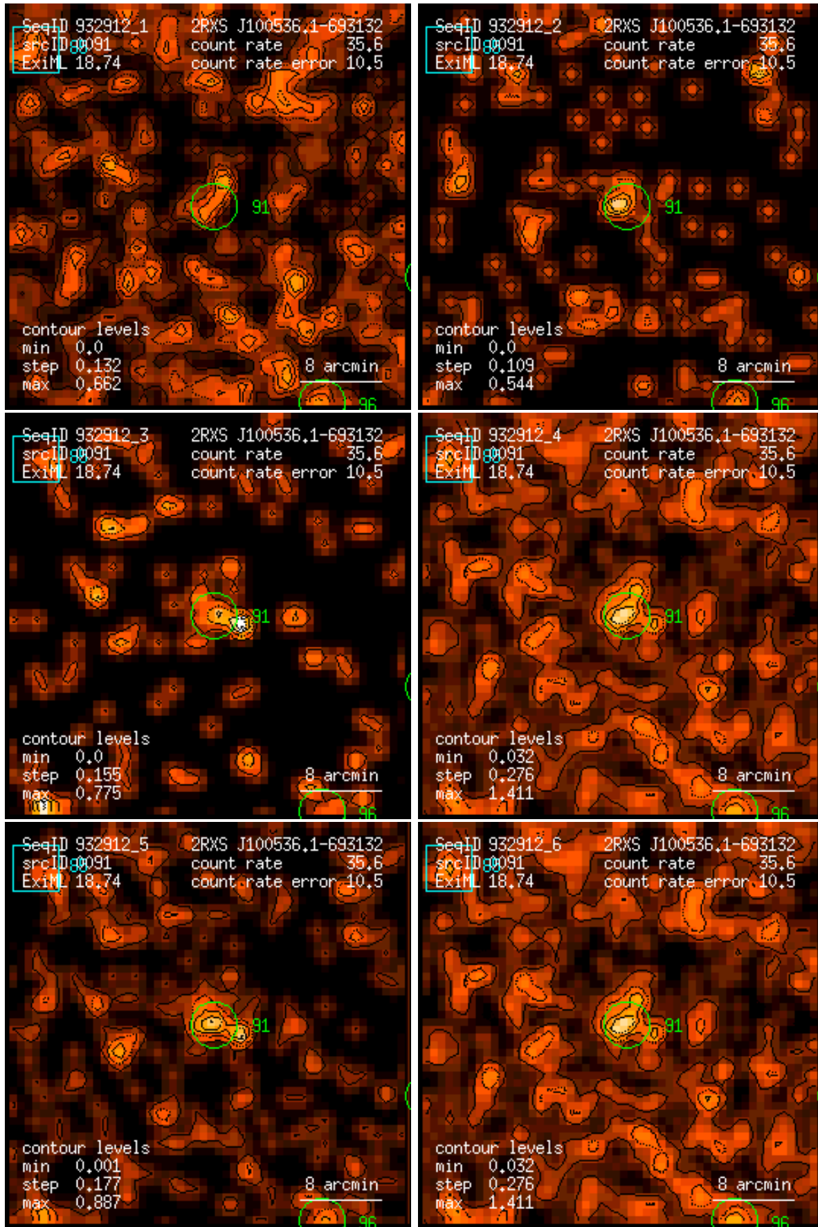
Figure 91: RASS 932912: detection 0091: band rate images, Gaussian filter: (1) PSPC channels 11 – 41, (2) 52 – 90, (3) 91 – 201, (4) 11 – 235, (5) 52 – 201, (6) 11 – 201. Broad band rates in counts/ks. Band rate contour levels in counts/ks/arcmin 2 .
