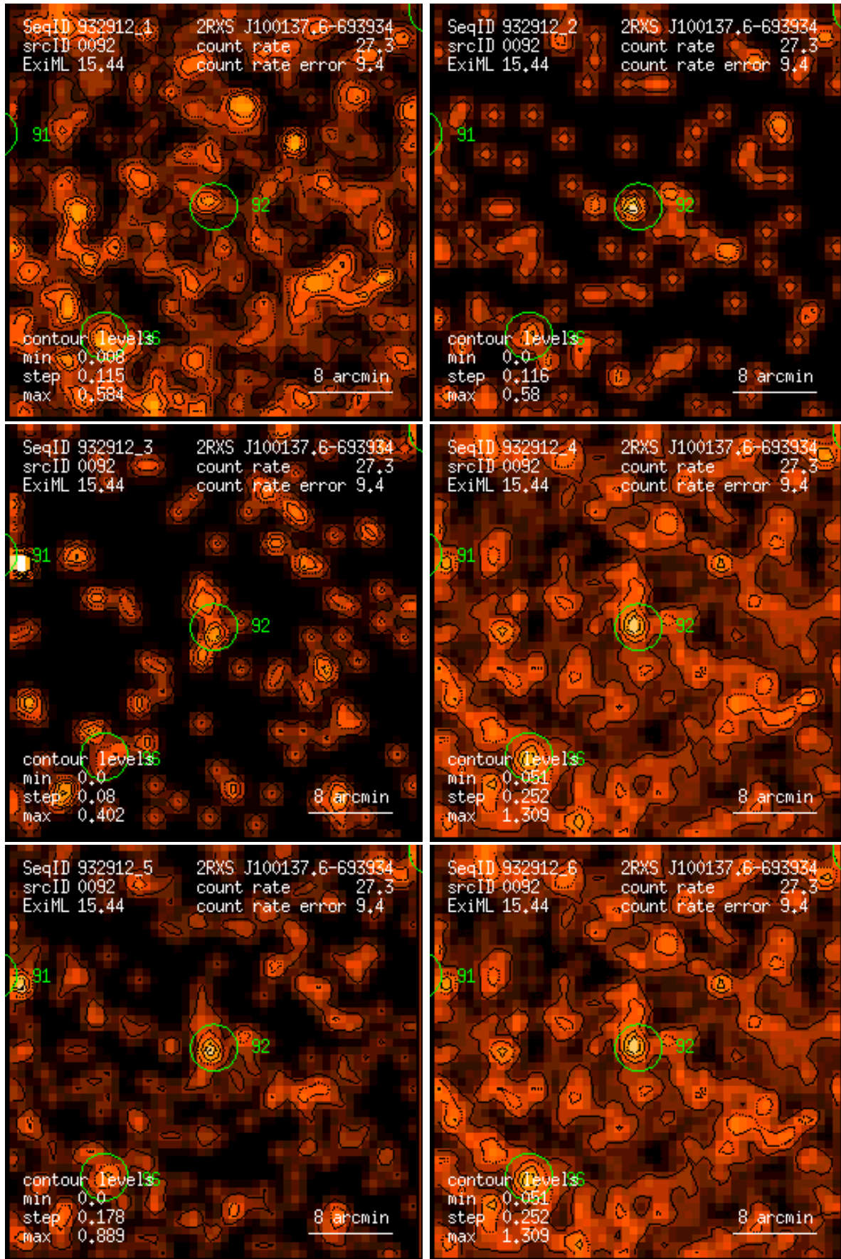
Figure 92: RASS 932912: detection 0092: band rate images, Gaussian filter: (1) PSPC channels 11 – 41, (2) 52 – 90, (3) 91 – 201, (4) 11 – 235, (5) 52 – 201, (6) 11 – 201. Broad band rates in counts/ks. Band rate contour levels in counts/ks/arcmin 2 .
